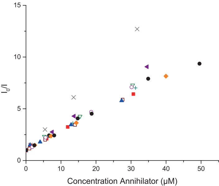
Fig. 5 Stern-Volmer plot of PtOEP (0.5 μM) phosphorescence quenching 1 (●), 2 (x), 3 (■), 4 (▲), 5 (◆), 6 (▽), 7 (+), 8 (▼), 9 (○) and 10 (□).
