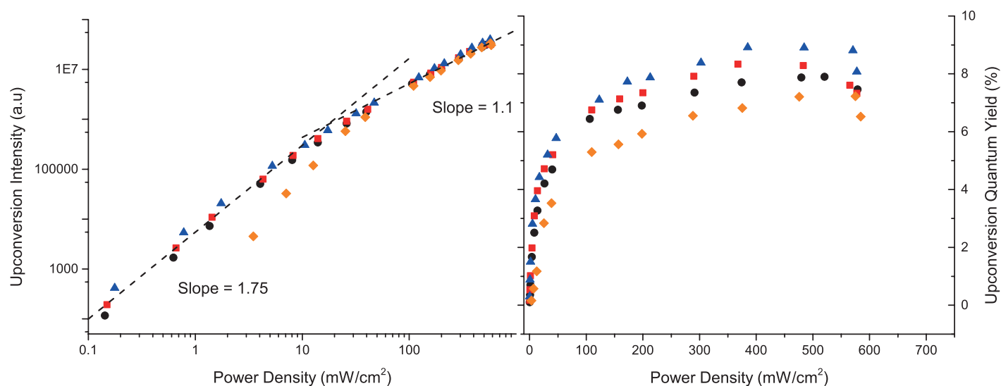
Fig. 7 Left: Double logarithmic plot of integrated upconverted emission dependence on excitation power density (532 nm) of solutions containing PtOEP , 15 \mu\text{M} and 0.5 mM annihilator. Right: Upconverted emission quantum yield ( \Phi_{UC} ) as a function of excitation power density of the same solutions. 1 ( \bullet ), 3 ( \blacksquare ), 4 ( \blacktriangle ) and 5 ( \blacklozenge ).
