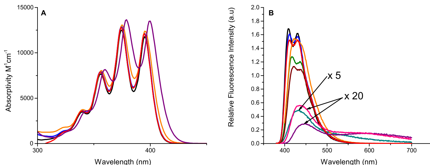
Fig. 4 a) Molar absorptivity of the representative compounds 1 (—), 3 (—), 4 (—), 5 (—), 8 (—) and b) Relative Fluorescence intensity of synthesized anthracene derivatives compared to 1 (—), 3 (—), 4 (—), 5 (—), 6 (—), 7 (—), 8 (—), 9 (—) and 10 (—), spectra are corrected for absorbance.
