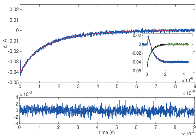
Fig. 6 Transient absorption measurements of 4 (1 mM) and PtOEP (3.4 \mu M) at 410 nm (Annihilator Decay, blue) and 650 nm (Sensitizer decay, black) and respective fits. Inset shows the first 5 \mu s. Bottom panel shows the residual of the fitted annihilator decay.
