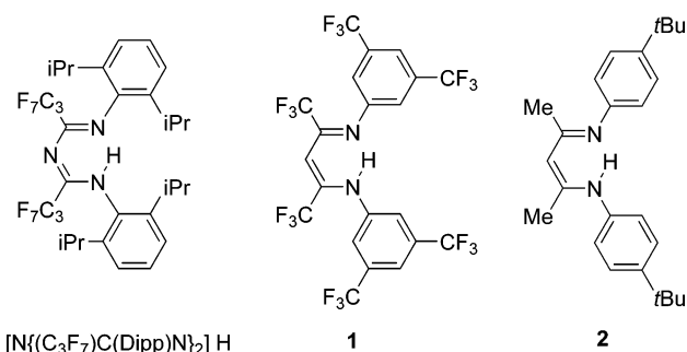
Figure 1. \beta -Diketimine ligands.
