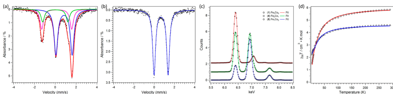
Figure 3. Zero-field ^{57}\text{Fe} Mössbauer spectrum obtained at 90 K and spectral fits ( \delta , |\Delta E_Q| (mm/s)) for (a) (\text{PhL})\text{Fe}_2\text{CoCl}(\text{NCCH}_3) ( 4 ; component 1 (blue): 0.83, 1.41, 56.7%; component 2 (green): -0.01 , 2.36, 22.1%; component 3 (magenta): 0.21, 2.92, 21.1%); (b) [(\text{PhL})\text{Co}_2\text{Fe}(\mu\text{-Cl})]_2 ( 6 ; 0.69, 1.38). (c) X-ray fluorescence spectra (data black circles, fits represented as lines): of 1 (red), 4 (green), 6 (blue). (d) Variable-temperature magnetic susceptibility data for 4 (circles) and 5 (triangles) collected in an applied dc field of 0.1 T. Solid lines represent fits to the data as described in the text.
