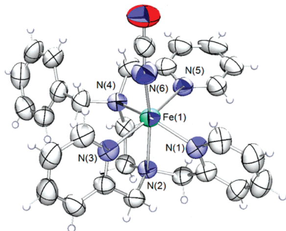
Figure 2. ORTEP diagram of the [\text{Fe}(\text{bztpen})\text{OCN}]\text{PF}_6 compound. The thermal ellipsoids are shown at 50% probability.
