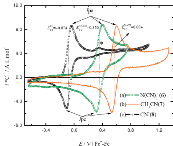
Figure 4. Typical cyclic voltammograms obtained for \sim 1.0 \text{ mM} (a) [\text{Fe}(\text{bztphen})\text{N}(\text{CN})_2]\text{PF}_6 , (c) [\text{Fe}(\text{bztphen})\text{CN}]\text{PF}_6 , and (b) [\text{Fe}(\text{bztphen})\text{CH}_3\text{CN}](\text{PF}_6)_2 in 0.1 \text{ M} of \text{Bu}_4\text{NPF}_6 acetonitrile solution at 100 \text{ mV s}^{-1} on a carbon glass electrode. In all cases, the potential scan was initiated in the positive direction from E_i=0 .
