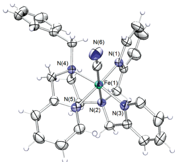
Figure 1. ORTEP diagram of the [\text{Fe}(\text{bztpen})\text{CN}]\text{PF}_6 compound. The thermal ellipsoids are shown at 50% probability.
