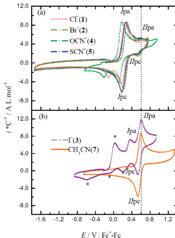
Figure 5. Typical cyclic voltammograms obtained for \sim 1.0 \text{ mM} of the (a) \text{Cl}^- , \text{Br}^- , \text{OCN}^- , and \text{SCN}^- derivatives and the (b) \text{I}^- and \text{CH}_3\text{CN} derivatives in 0.1 \text{ M} \text{Bu}_4\text{NPF}_6 acetonitrile solution at 100 \text{ mV s}^{-1} on a carbon glass electrode. In all cases, the potential scan was initiated in the positive direction from E_i=0 .
