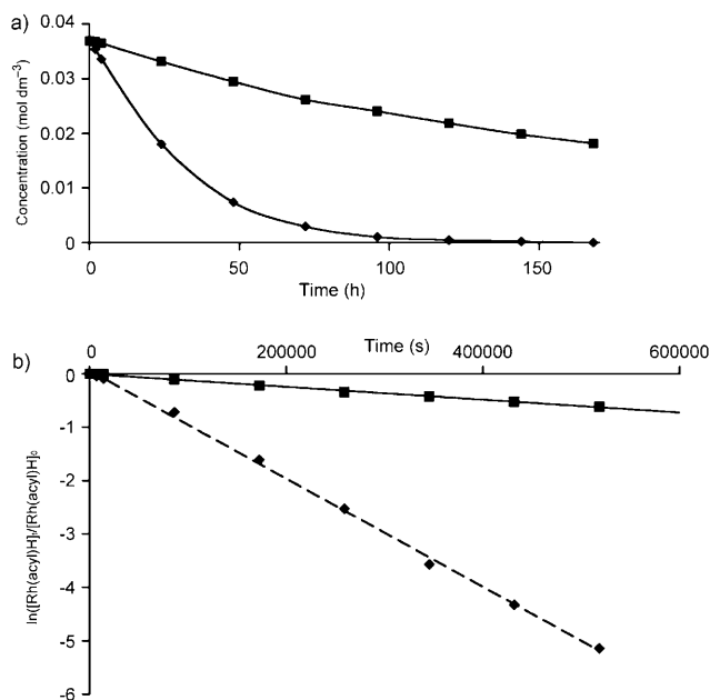
Figure 5. a) Decomposition of the acyl-hydride intermediates over one week. Concentrations calculated from NMR spectroscopic integrals by using an internal standard. b) Plot of \ln([Rh(acyl)hydride]/[Rh(acyl)hydride]_0) versus time to obtain rate constant, k , for the decomposition of the acyl-hydride complexes of the DPEphos ligand. ♦: 6a [CbCl 6 ]; ■: 6b [CbCl 6 ].
