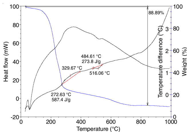
Fig. 3. TG/DTA curve of [\text{VO}(\text{AVOP})]\text{SO}_4 in static air
