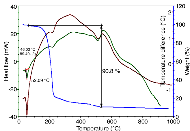
Fig. 4. TG/DTA curve of [\text{VO}(\text{AFOP})]\text{SO}_4 in static air
