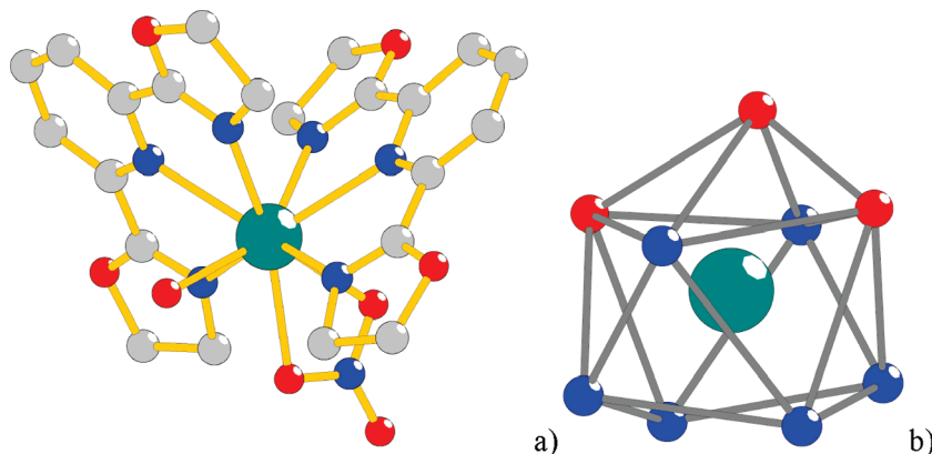
Figure 9. Ball-and-stick representations of (a) 6 , the 2:1 complex of Pybox with Tb(NO 3 ) 3 and (b) the distorted monocapped square antiprism coordination polyhedron around Tb(III). Hydrogen atoms, nitrate counterions, and methanol molecules of crystallization have been omitted for clarity.
