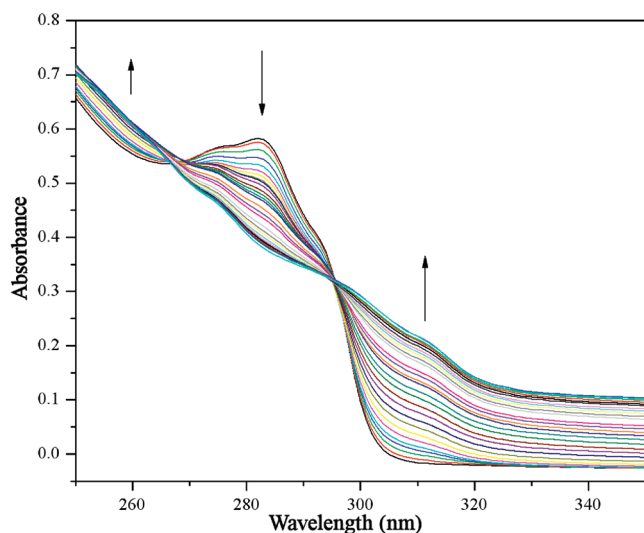
Figure 10. Absorption titration experiment of Pybox in acetonitrile with Tb(NO 3 ) 3 performed at constant ionic strength I = 0.1 M (Et 4 NCl); [Ln(Pybox) 3 ] 3+ = 1 × 10 −4 M.
