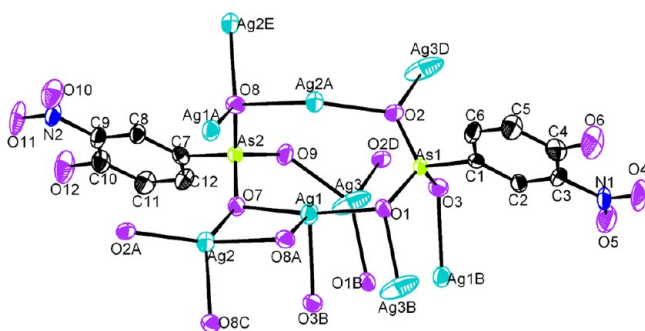
Figure 7. ORTEP representation of the selected unit in compound 3 . The thermal ellipsoids are drawn at 50% probability level. Symmetry codes for the generated atoms: (a) -x, -y, -z+1 ; (b) -x, -y+1, -z+1 ; (c) x+1, y, z ; (d) -x-1, -y+1, -z+1 ; (e) x-1, y, z .
