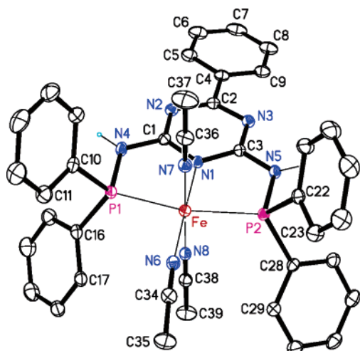
Figure 8. Structural view of [\text{Fe}(\text{PNP}^{\text{T-Ph}})(\text{CH}_3\text{CN})_3](\text{BF}_4)_2 \cdot 3\text{ClCH}_2\text{CH}_2\text{Cl} \cdot \text{H}_2\text{O} ( 11 · 3\text{ClCH}_2\text{CH}_2\text{Cl} \cdot \text{H}_2\text{O} ) showing 40% thermal ellipsoids (C-bonded H atoms, \text{BF}_4^- and solvent molecules omitted for clarity). Selected bond lengths ( \text{\AA} ) and bond angles (deg): Fe–P(1) 2.2430(4), Fe–P(2) 2.2409(4), Fe–N(1) 1.957(1), Fe–N(6) 1.942(1), Fe–N(7) 1.914(1), Fe–N(8) 1.915(1), P(1)–N(4) 1.707(1), P(2)–N(5) 1.702(1), N(4)–C(1) 1.355(2), N(5)–C(3) 1.353(2); P(1)–Fe–P(2) 165.44(2).
