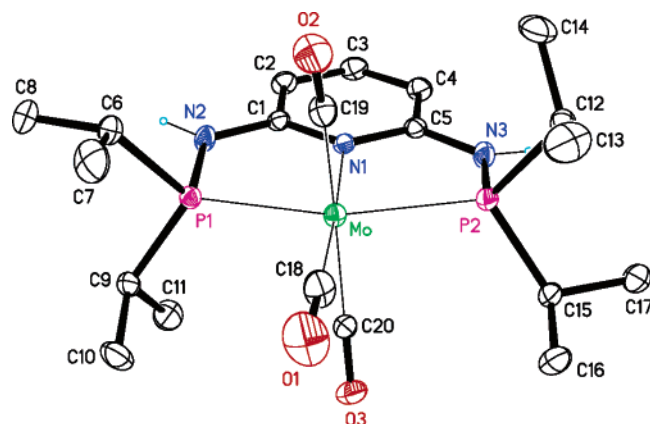
Figure 1. Structural view of Mo(PNP-Pr i )(CO) 3 ·CH 3 CN ( 4a ·CH 3 CN) showing 30% thermal ellipsoids (C-bonded H atoms and CH 3 CN omitted for clarity). Selected bond lengths (Å) and bond angles (deg): Mo–C(18) 1.948(1), Mo–C(19) 2.001(2), Mo–C(20) 2.024(1), Mo–N(1) 2.251(1), Mo–P(1) 2.4206(3), Mo–P(2) 2.3986(3); P(1)–Mo–P(2) 155.62(1), C(19)–Mo–C(20) 166.03(5).
