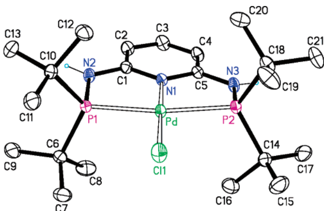
Figure 14. Structural view of [\text{Pd}(\text{PNP-Bu}^i)\text{Cl}]\text{Cl}\cdot 2\text{CH}_2\text{Cl}_2 ( 18c · 2\text{CH}_2\text{Cl}_2 ) showing 30% thermal ellipsoids (C-bonded H atoms, \text{CH}_2\text{Cl}_2 , and \text{Cl}^- omitted for clarity). Selected bond lengths (Å) and bond angles (deg): Pd–P(1) 2.2987(5), Pd–P(2) 2.2985(5), Pd–N(1) 2.015(2), Pd–Cl(1) 2.3002(6), P(1)–Pd–P(2) 166.54(2).
