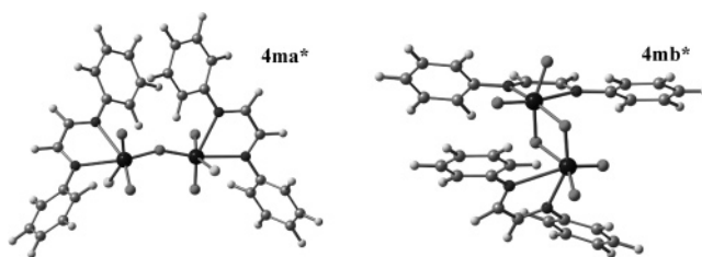
Figure 5. DFT-optimized geometries of two possible Mo(VI) dimers [\{\text{MoO}_2\text{Cl}(\text{N-N})\}_2(\mu\text{-O})] ( 4ma* ) and [\{\text{MoO}_2(\text{N-N})\}_2(\mu\text{-O})_2] ( 4mb* ).
