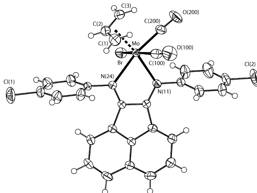
Figure 1. ORTEP diagram showing the molecular structure of [\text{Mo}(\eta^3\text{-C}_3\text{H}_5)\text{Br}(\text{CO})_2\{1,4\text{-(4-chloro)phenyl-2,3-naphthalenediazabutadiene}\}] ( 7 ) with thermal ellipsoids drawn at 50% probability level.
