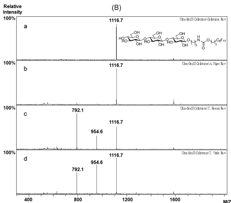
Figure 4. Study of cellulase activity using glycan array combined with mass spectrometry. (A) Hydrolyzed fragments of cellotriose derivatives remained on the Teflon-like ACG slide surface. (B) MS-TOF data of enzymatic hydrolysis of polyfluorinated cellotriose of the control run without enzymes (a), and with the cellulase proteins from A. niger (b), T. reesei (c), and A. viride (d).
