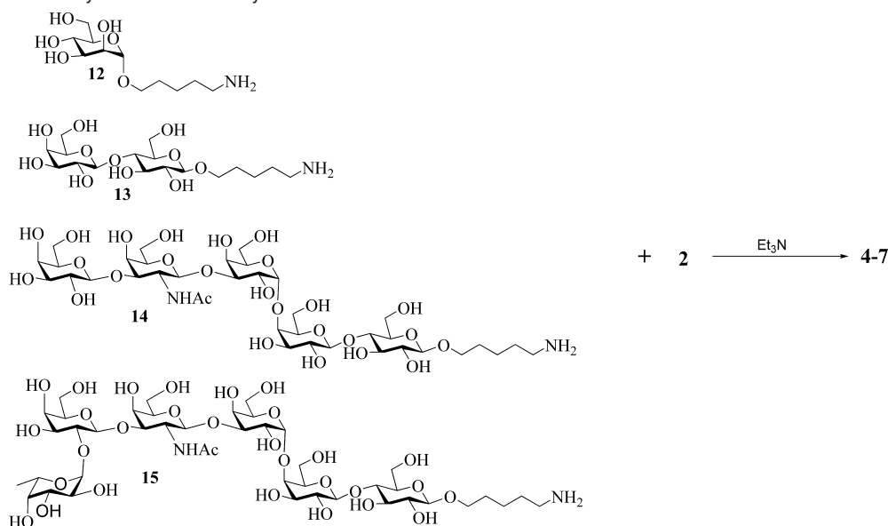
Scheme 1. Synthesis of Polyfluorinated Carbohydrates 4–7
