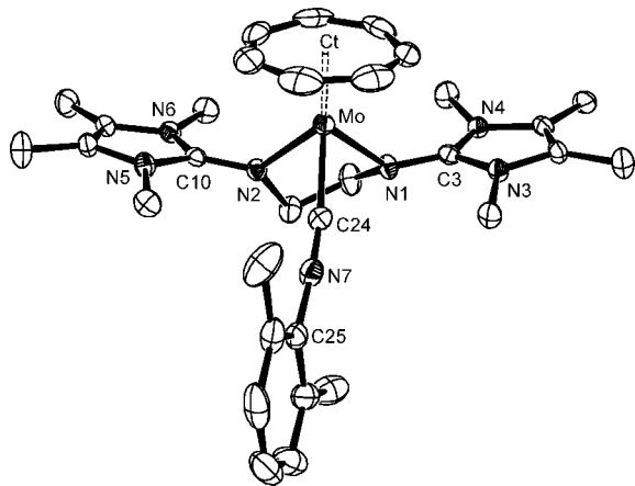
Figure 6. ORTEP drawing of the cation in [2(\text{CNXy})]\text{PF}_6 with thermal displacement parameters drawn at 50% probability. Selected bond lengths [Å] and angles [deg]: Mo–N1 2.252(3), Mo–N2 2.189(3), Mo–C24 2.077(3), Mo–C(Ch) 2.271(4)–2.324(4), N1–C3 1.326(4), N2–C10 1.327(4), C24–N7 1.172(5), N1–Mo–N2 76.7(1), Mo–C24–N7 173.5(3), C24–N7–C25 174.3(4).
