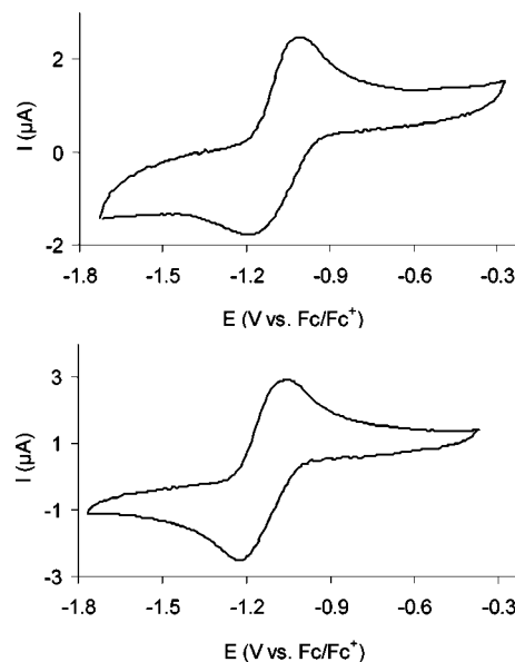
Figure 3. Cyclic voltammetric traces of [1]\text{BF}_4 (above) and [2]\text{PF}_6 (below), 1.0 mM solution in acetonitrile, (TBA)PF 6 (0.1 M), scan rate 0.1 V/s, T = 25^\circ\text{C} , against a Ag/AgCl reference electrode (3 M KCl), Pt working electrode; the ferrocene/ferrocenium couple displays a redox potential E^\circ = +476 mV, and the values are referenced to E^\circ(\text{Fc}/\text{Fc}^+) = 0 mV.
