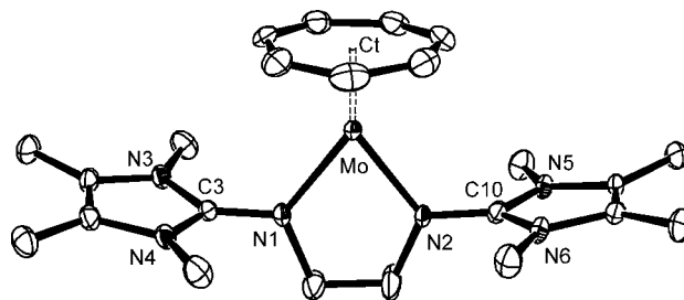
Figure 2. ORTEP drawing of the cation in [2]\text{BF}_4 \cdot \text{CH}_3\text{CN} with thermal displacement parameters drawn at 50% probability. Selected bond lengths [Å] and angles [deg]: Mo–N1 2.076(3), Mo–N2 2.063(3), Mo–C(Cht) 2.226(4)–2.307(4), N1–C3 1.357(4), N2–C10 1.363(4); N1–Mo–N2 76.5(1).
