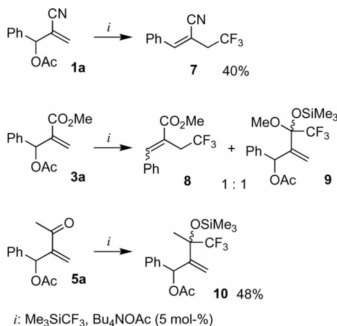
Scheme 2. Trifluoromethylation reactions.
