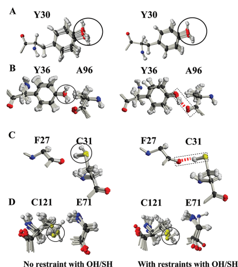
Figure 7. The 10 lowest energy structures of SAIL-EPPIbEPPIb, superimposed for the regions including Tyr-30 (A), Tyr-36 (B), Cys-31 (C), and Cys-121 (D). For each panel, structures determined without (left) and with (right) distance restraints with OH/SH are shown. For clarity, conformers were again superimposed for each displayed region. Side-chain hydroxyl and sulfhydryl groups are circled or, when hydrogen bonds are explicitly formed, enclosed by a dashed box together with its hydrogen-bond acceptor atom.
