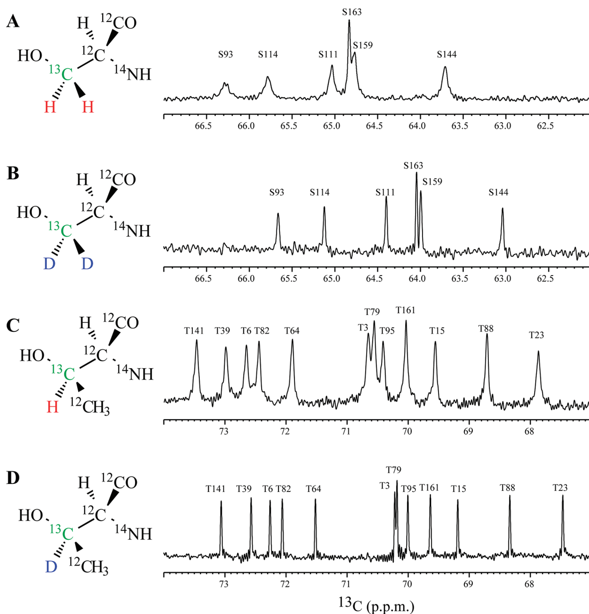
Figure 2. 150.9 MHz ^2\text{H}, ^1\text{H} -decoupled 1D ^{13}\text{C} NMR spectrum of EPPIb, selectively labeled with L- [\beta\text{-}^{13}\text{C}] serine (A), L- [\beta\text{-}^{13}\text{C}; \beta, \beta\text{-}^2\text{H}] serine (B), L- [\beta\text{-}^{13}\text{C}] threonine (C), and L- [\beta\text{-}^{13}\text{C}; \beta, \beta\text{-}^2\text{H}] threonine (D). These spectra were acquired at 40 °C at 150.9 MHz of ^{13}\text{C} frequency. In (B) and (D), proton and deuterium decoupling was applied during acquisition. The chemical shift differences between L- [\beta\text{-}^{13}\text{C}] serine and L- [\beta\text{-}^{13}\text{C}; \beta, \beta\text{-}^2\text{H}] serine and those between L- [\beta\text{-}^{13}\text{C}] threonine and L- [\beta\text{-}^{13}\text{C}; \beta, \beta\text{-}^2\text{H}] threonine are due to the deuterium isotope shift effect arising from the proton/deuterium substitution of methylene protons. Each peak is labeled with its assignment.
