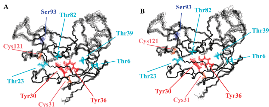
Figure 5. The 20 solution structures of SAIL-EPPIb, determined without (A) and with (B) distance restraints involving observable hydroxyl/sulfhydryl protons, superimposed on a well-defined region (a.a. 1–87, 92–110, 118–136, and 153–162). The side-chains of the Ser, Thr, Cys, and Tyr residues are colored blue, cyan, orange, and red, respectively.
