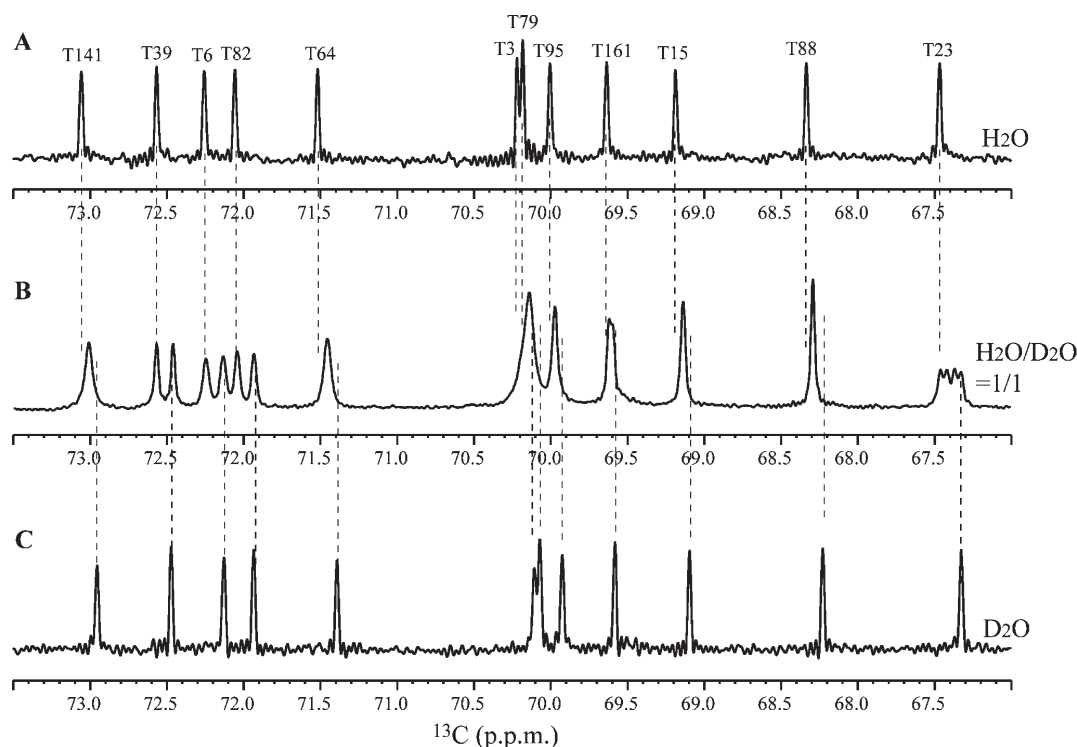
Figure 4. 150.9 MHz [^2\text{H}, ^1\text{H}] -decoupled 1D ^{13}\text{C} NMR spectra of EPPIb, selectively labeled with L- [\beta\text{-}^{13}\text{C}; \beta\text{-}^2\text{H}] threonine in \text{H}_2\text{O} (A), \text{H}_2\text{O}/\text{D}_2\text{O} (1:1) (B), and \text{D}_2\text{O} (C) buffers. Sample concentrations were 0.2–0.7 mM, and all experiments were performed at 40 °C. Peaks are labeled with their assignments. The ^{13}\text{C}_\beta resonances for Thr-6, Thr-39, and Thr-82 were observed as two signals in an \text{H}_2\text{O}/\text{D}_2\text{O} (1:1) buffer, due to the isotope effect from the side-chain hydroxyl groups. The ^{13}\text{C}_\beta resonance for Thr-23 was observed as the four-line signals in \text{H}_2\text{O}/\text{D}_2\text{O} (1:1), due to the dual isotope effect from the backbone amide and side-chain hydroxyl groups.
