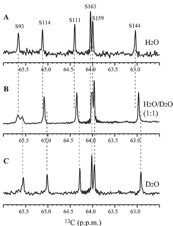
Figure 3. 150.9 MHz [^2\text{H}, ^1\text{H}] -decoupled 1D ^{13}\text{C} NMR spectra of EPPIb, selectively labeled with L - [\beta\text{-}^{13}\text{C}; \beta, \beta\text{-}^2\text{H}_2] serine. The labeled EPPIb was dissolved in \text{H}_2\text{O} (A), \text{H}_2\text{O}/\text{D}_2\text{O} (1:1) (B), and \text{D}_2\text{O} (C) buffers to concentrations ranging from 0.2 to 0.7 mM for each solution at pH 7.5. Peaks are labeled with their assignments. These NMR experiments were performed at 40 °C. The ^{13}\text{C}_\beta resonances for Ser-93 were observed as two signals in an \text{H}_2\text{O}/\text{D}_2\text{O} (1:1) buffer, due to the isotope effect from the side-chain hydroxyl groups. Overall, the line-width of each peak in an \text{H}_2\text{O}/\text{D}_2\text{O} (1:1) buffer is slightly larger than that in \text{H}_2\text{O} or \text{D}_2\text{O} , due to the unresolved isotope effect from the backbone amide group.
