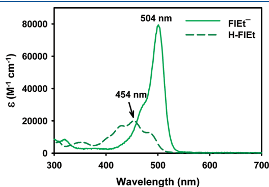
Figure 1. Electronic absorption spectra of fluorescein ethyl ester ( FIEt , in 50:50 MeCN/ \text{H}_2\text{O} ) and protonated FIEt-H (in MeCN/ \text{AcOH} pH = 5).
