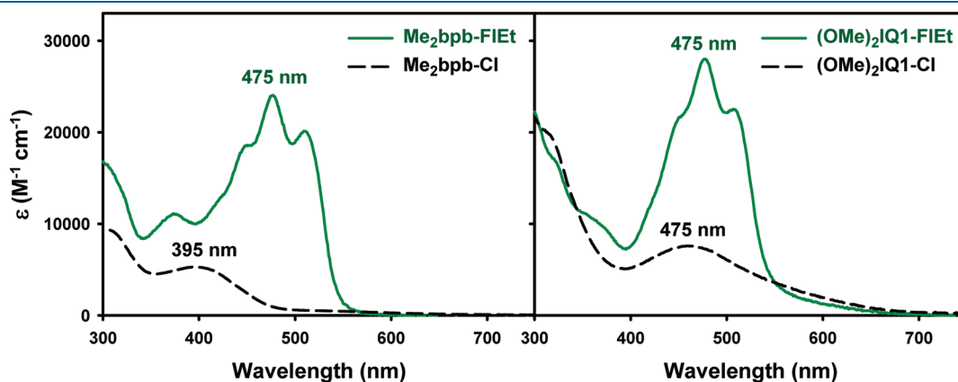
Figure 2. Electronic absorption spectra of [(\text{Me}_2\text{bpb})\text{Ru}(\text{NO})(\text{Cl})] and [(\text{Me}_2\text{bpb})\text{Ru}(\text{NO})(\text{FIEt})] (left panel) and [((\text{OMe})_2\text{IQ1})\text{Ru}(\text{NO})(\text{Cl})] and [((\text{OMe})_2\text{IQ1})\text{Ru}(\text{NO})(\text{FIEt})] (right panel) in MeCN.
