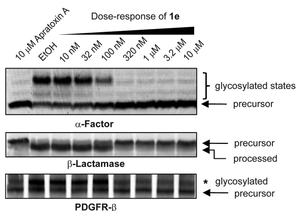
Figure 3. Apratoxin S4 ( 1e ) inhibits cotranslational processing in vitro. Products of in vitro translation reactions (rabbit reticulocyte, amino acids, [ ^{35} S]methionine, canine pancreatic microsomal membranes, mRNA template, and apratoxin 1e ) were separated by SDS-PAGE to autoradiographically detect effects on translation and glycosylation of \alpha -factor and signal peptide cleavage of \beta -lactamase. When PDGFR- \beta cDNA was used as a template, in vitro transcription/translation was carried out using T7 TNT Quick Master Mix and glycosylation determined by SDS-PAGE followed by autoradiography.
