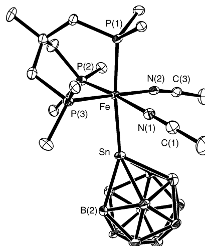
Figure 1. Molecular structure of [1-{Fe(MeCN) 2 (triphos)}-SnB 11 H 11 ] (1). The hydrogen atoms and the phenyl rings except the ipso -carbon atoms have been omitted for clarity. Selected bond distances [Å] and angles [deg]: C(1)–N(1) 1.132(7), C(3)–N(2) 1.134(7), B(2)–Sn 2.310(6), B(3)–Sn 2.327(5), B(4)–Sn 2.329(6), B(5)–Sn 2.343(6), B(6)–Sn 2.329(6), N(1)–Fe 1.953(4), N(2)–Fe 1.942(4), Fe–P(1) 2.264(1), Fe–P(2) 2.249(1), Fe–P(3) 2.276(1), Fe–Sn 2.587(1), N(2)–Fe–N(1) 83.63(17), N(1)–Fe–P(1) 96.96(13), N(1)–Fe–P(2) 171.43(13), N(1)–Fe–P(3) 93.43(13), P(2)–Fe–P(1) 90.26(5), P(2)–Fe–P(3) 91.67(5), P(1)–Fe–P(3) 86.11(5), N(1)–Fe–Sn 80.60(12), N(2)–Fe–Sn 79.85(11), P(1)–Fe–Sn 172.96(5), P(2)–Fe–Sn 91.70(4), P(3)–Fe–Sn 100.59(4).
