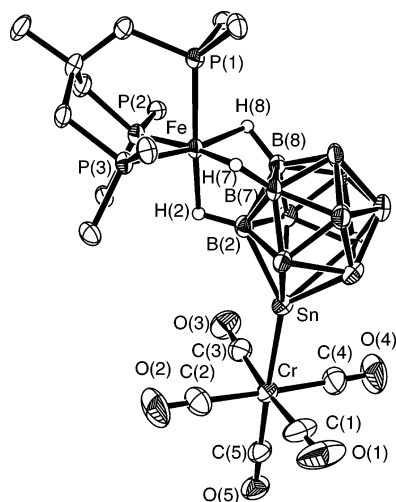
Figure 3. Molecular structure of [1-\{\text{Cr}(\text{CO})_5\}-2,7,8-(\mu\text{-H})_3-\{\text{Fe}(\text{triphos})\}-\text{SnB}_{11}\text{H}_{11}] , 3 . The hydrogen atoms and the phenyl rings except the ipso -carbon atoms have been omitted for clarity.
