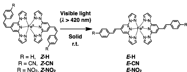
Scheme 1. Photoisomerization from the Z-Form to the E-Form upon Visible Light ( \lambda > 420 nm) Irradiation in Fe II Complexes Studied a
