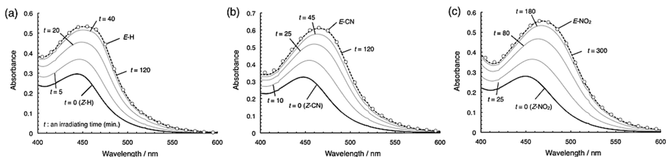
Figure 2. UV-vis spectral changes of (a) Z-H, (b) Z-CN, and (c) Z-NO 2 in acetonitrile upon irradiation with 436 nm light. The spectra of the corresponding E -form complexes are indicated by black circles, and the concentrations of the complexes were 1.0 \times 10^{-4} M.
