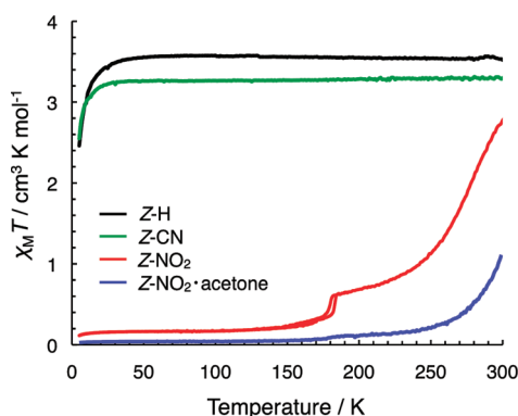
Figure 9. Temperature dependence of \chi_M T for Z-H, Z-CN, Z- \text{NO}_2 , and Z- \text{NO}_2 ·acetone in the microcrystalline state.
