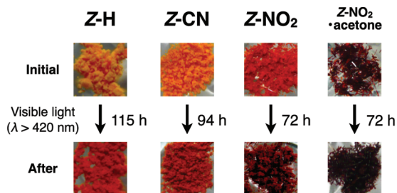
Figure 4. Color changes of the microcrystalline Z-H, Z-CN, Z-NO 2 , and Z-NO 2 ·acetone upon irradiation with visible light ( \lambda > 420 nm) for 115 h in Z-H, 94 h in Z-CN, and 72 h in Z-NO 2 and Z-NO 2 ·acetone.
