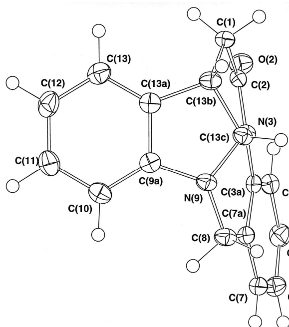
Figure 3. Molecular projection of 7a normal to the phenyl ring
