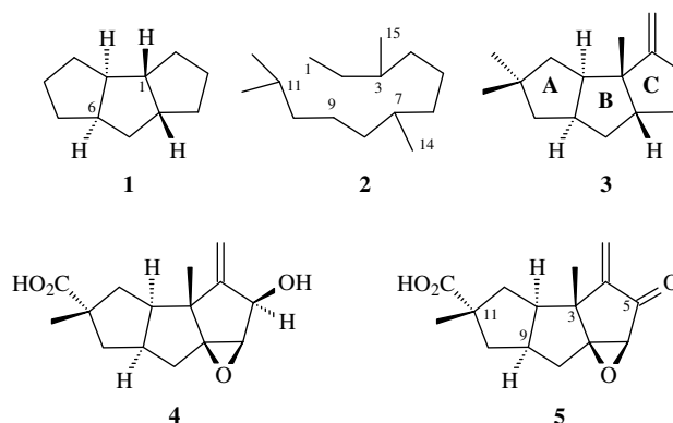
Fig. 1. Linear triquinane frameworks.
