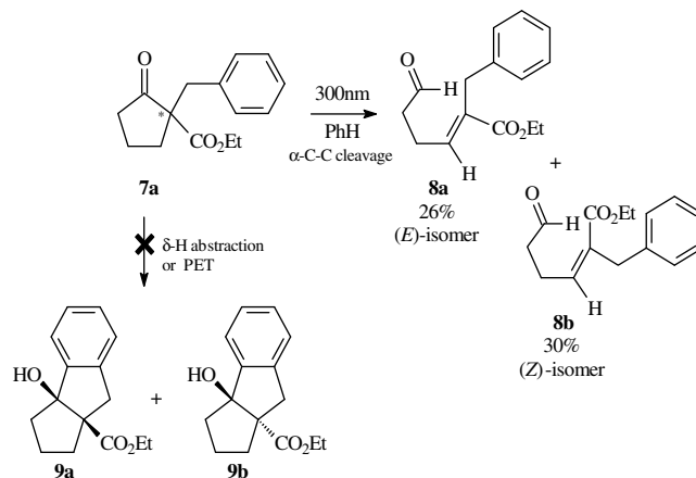
Scheme 2. Photoinduced \alpha -C–C cleavage of 7a .
