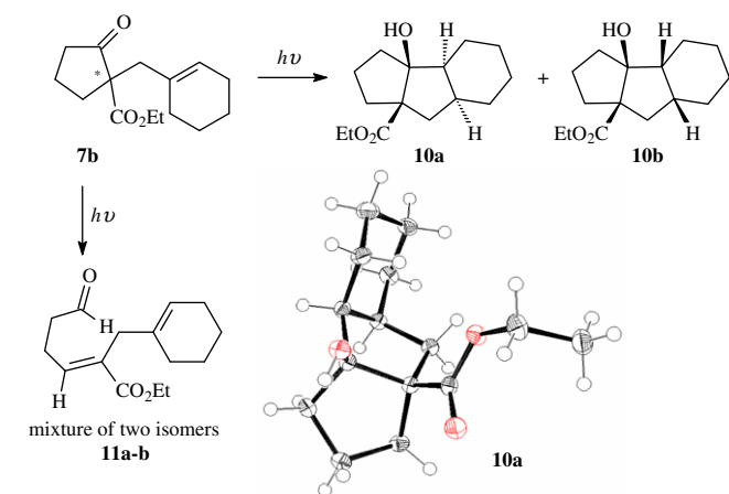
Scheme 3. Photoinitiated reactions of 7b .
