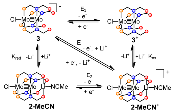
Scheme 2. Square Scheme for the Electrochemistry of Complexes 2-MeCN and 3
