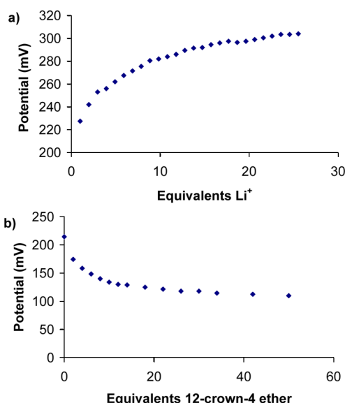
Figure 6. Potential of the MeCN solution of 2-py as a function of (a) the equivalents of \text{Li}^+ added and (b) the equivalents of 12-crown-4 added. All potentials are referenced to the \text{Fc}/\text{Fc}^+ redox couple.
