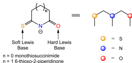
Chart 2. Ligands Monothiosuccinimide and 6-Thioxo-2-piperidinone
