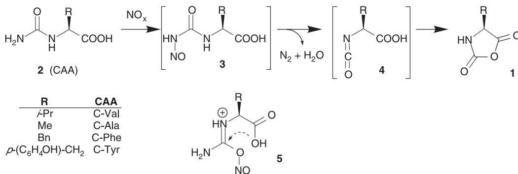
Scheme 2
