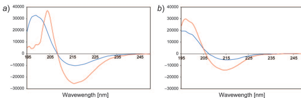
Fig. 2. Normalized CD spectra of the linear \beta -peptide 1 (blue) and the tethered \beta -peptide 4 (red) in MeOH (a), and in H 2 O (b; pH 7.1)
