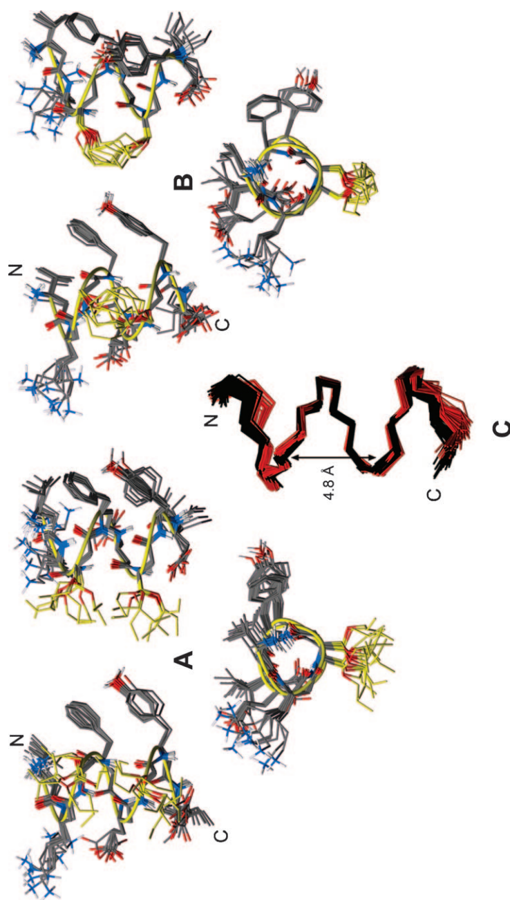
Fig. 5. Superposition of the structures of \beta -octapeptides 1 and 4 . A and B : The ten lowest-energy structures of 1 and 4 . Superposition was carried out over backbone atoms N, C, C ^\alpha , and C ^\beta of residues 2–7. Each bundle is shown from three different perspectives (front view, side view (rotated by 60^\circ ), and top view). In each bundle, a yellow ribbon through atoms C ^\beta in residues 1–8 of the structure lowest in energy indicates the backbone of the 3_{14} -helix. The side chains of residues 3 and 6 ( \beta^3 hSer(All) in 1 and bridge in 4 ) are also colored yellow. C- and N-termini of the sequences are indicated by the letters C and N. C : Superposition of all 45 structures of 1 and of 4 (red). Superposition was carried out over atoms N, C, C ^\alpha , and C ^\beta of residues 2–7. Only the backbone is shown. The average C ^\beta ...C ^\beta distance within the helices is ca. 4.8 Å (pitch of the helix).
