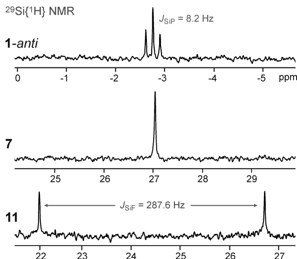
Figure 4. ^{29}\text{Si}\{^1\text{H}\} NMR spectra of complexes 1-anti , 7 , and 11 .
