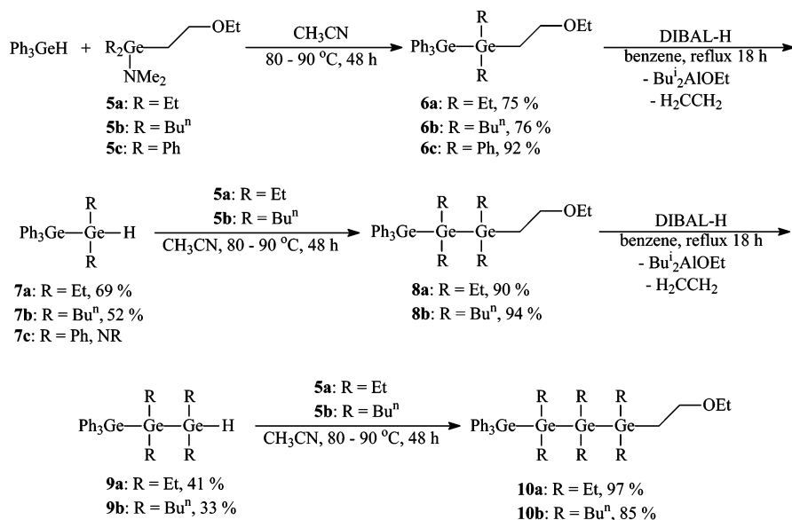
Scheme 4
