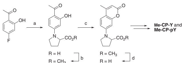
Scheme 2. Reagents and conditions: (a) L- or D-proline, K_2CO_3 , DMSO, \Delta , 99%; (b) CH_3I , K_2CO_3 , DMF, 93%; (c) Ph_3P=CHCO_2CH_3 , Ph_2O , \Delta , 78%; (d) LiOH , H_2O , THF, 78%.
