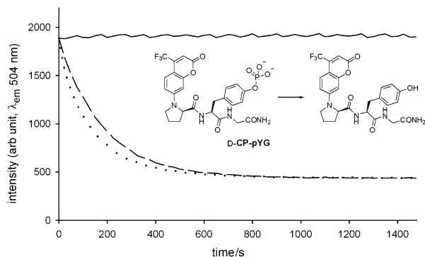
Figure 2. Fluorescence changes during phosphatase-catalyzed reactions (solid, no enzyme; dashed, phosphatase from potato; dotted, phosphatase from wheat germ). [D-CP-pYG]_0 = 1 \mu M and [enzyme] = 6 U L^{-1} in 50 mM citric acid buffer (pH 5.0) with 1% MeOH, \lambda_{ex} = 390 nm .
