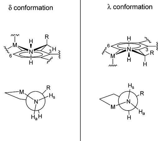
Scheme 6. Conformations of the Five-Membered Metallacycles in Complexes 8–12, 18, and 19; R = Me or Et; M = Ru or Rh
