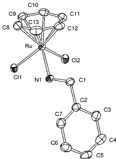
Figure 2. ORTEP style plot of compound 16 . Thermal ellipsoids are drawn at the 50% probability level, and hydrogen atoms are omitted for clarity. Selected bond lengths [Å] and bond angles [deg]:
