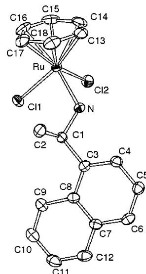
Figure 1. ORTEP style plot of compound 15 . Thermal ellipsoids are drawn at the 50% probability level, and hydrogen atoms are omitted for clarity. Selected bond lengths [Å] and bond angles [deg]: Ru–N 2.164(2), Ru–Cl1 2.4114(7), Ru–Cl2 2.4191(7), Ru–Centroid 1.651(3), N–Ru–Cl1 89.35(7), N–Ru–Cl2 82.74(7), Cl1–Ru–Cl2 86.80(3), N1–Ru–Centroid 128.57(15).
