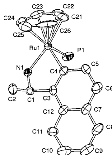
Figure 4. ORTEP style plot of one of the two inequivalent molecules of (R C ,S Ru )- 12 . Thermal ellipsoids are drawn at the 50% probability level, and hydrogen atoms, PF 6 , and substituents of PMe 2 Ph are omitted for clarity. Selected bond lengths [Å] and bond angles [deg]: Ru1–Centroid 1.734(8), Ru1–C4 2.068(7), Ru1–N1 2.139(5), Ru1–P1 2.3090(18), C4–Ru1–N1 77.7(2), C4–Ru1–P1 83.7(2), N1–Ru1–P1 88.81(16), N1–Ru1–Centroid 130.21(4).
