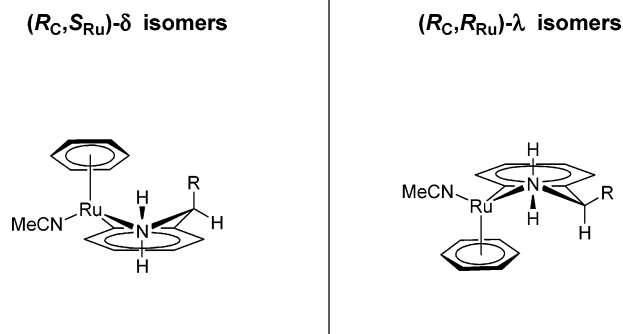
Scheme 9. Diastereoisomers of Complexes 13 (L = MeCN) and 14 (L = PMe 2 Ph) a
