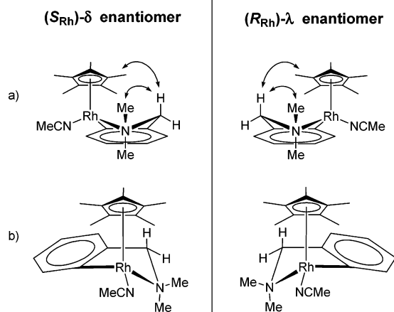
Scheme 5. Conformations of Complex 17: (a) Front Views; (b) Side Views a
