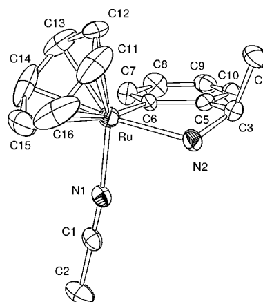
Figure 3. ORTEP style plot of compound (R C ,S Ru )- 8 . Thermal ellipsoids are drawn at the 50% probability level, and hydrogen atoms are omitted for clarity. Selected bond lengths [Å] and bond angles [deg]: Ru–Centroid 1.698 (6), Ru–N1 2.066(4), Ru–N2 2.120(4), Ru–C6 2.064(4), N1–Ru–N2 85.6(1), N1–Ru–C6 86.3(1), N2–Ru–C6 78.2(2), N2–Ru–Centroid 132.59(4).
