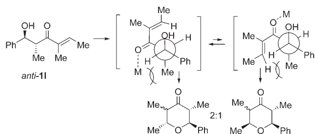
Scheme 10. Cyclisation of anti -aldol 11 .
