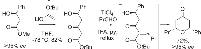
Scheme 1. Representative approaches towards tetrahydropyranones. TBAF = tetrabutylammonium fluoride; TFA = trifluoroacetic acid; de = diastereomeric excess.
