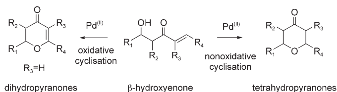
Scheme 2. \text{Pd}^{\text{II}} -mediated oxidative and nonoxidative ring closure of \beta -hydroxyenones.
