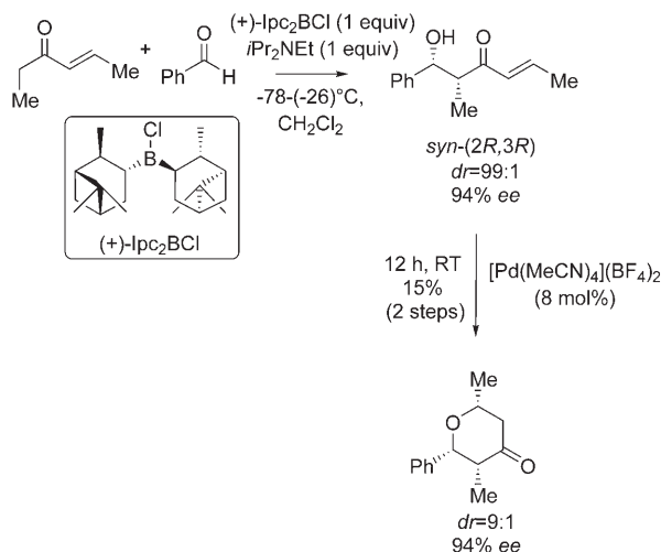
Scheme 4. Asymmetric synthesis of (2 R ,3 R ,6 R )-2-phenyl-3,6-dimethyltetrahydropyran-4-one 2k .
