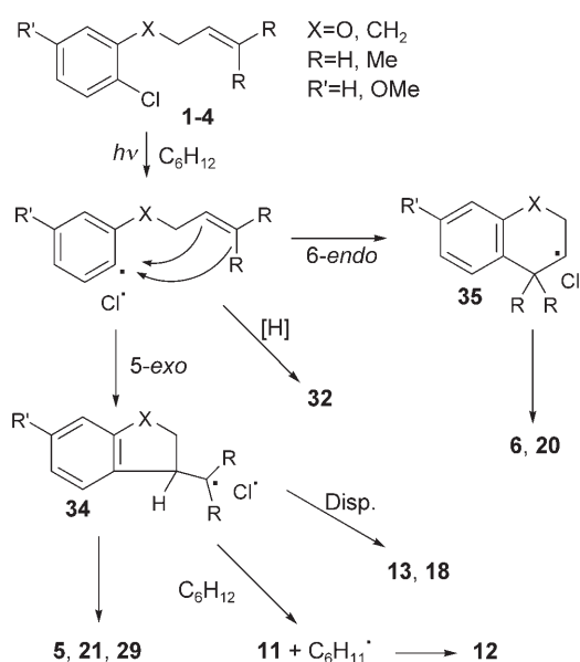
Scheme 6. Radical pathways after photolysis of compounds 1–4 .
