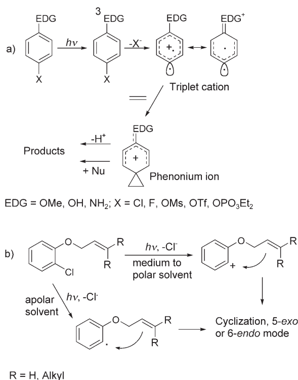
Scheme 1. a) Interolecular and b) proposed intramolecular chemistry of phenyl cations.
