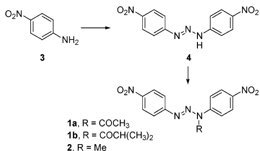
SCHEME 1. Synthesis of Triazenes 1 and Reference Compound 2
