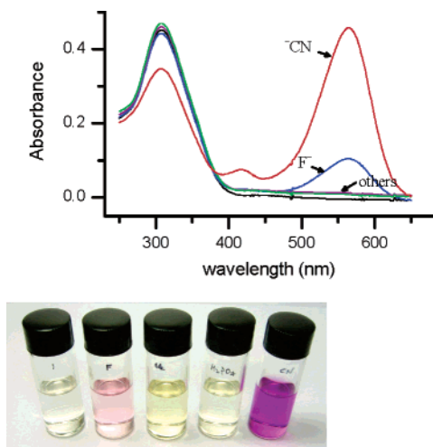
FIGURE 4. Absorption spectra and corresponding color changes when triazene 1b (0.017 mM) was treated with selected anions (vials from the left: 1b only, \text{F}^- , \text{AcO}^- , \text{H}_2\text{PO}_4^- , and \text{CN}^- as \text{Bu}_4\text{N}^+ salts; 1.15 equiv) in \text{CH}_3\text{CN} .
