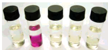
FIGURE 5. A two-phase detection experiment with triazene 1a (0.5 mM) in the presence of a phase-transfer catalyst ( \text{Bu}_4\text{N}^+\text{Br}^- , 0.1 M) in \text{CH}_2\text{Cl}_2 -Tris buffer (pH 8.6, 1.0 mM) with selected anions (from the left: 0.5 mL of 1a only, NaCN, NaOAc, \text{NaH}_2\text{PO}_4 , and KF).
