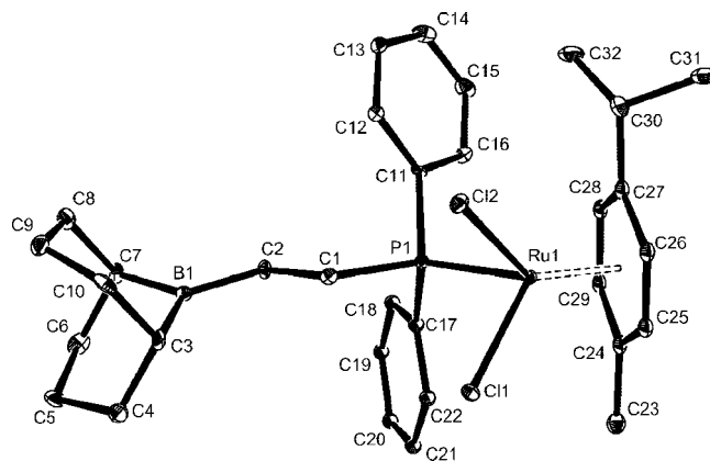
Figure 1. Molecular view of 2b in the solid state (thermal ellipsoids at the 30% probability level), with hydrogen atoms and solvate molecules omitted. Selected bond lengths (Å) and bond angles (deg): \text{P1}\text{---}\text{Ru1} = 2.352(2) , \text{Ru1}\text{---}\text{Cl1} = 2.4003(19) , \text{Ru1}\text{---}\text{Cl2} = 2.4106(18) , \text{P1}\text{---}\text{C1} = 1.841(7) , \text{C1}\text{---}\text{C2} = 1.526(9) , \text{C2}\text{---}\text{B1} = 1.565(11) ; \text{Cl1}\text{---}\text{Ru1}\text{---}\text{Cl2} = 86.73(7) , \text{P1}\text{---}\text{Ru1}\text{---}\text{Cl1} = 87.72(7) , \text{P1}\text{---}\text{Ru1}\text{---}\text{Cl2} = 85.78(7) .
