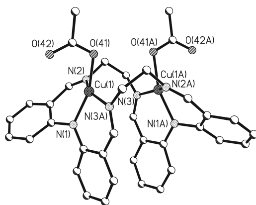
Figure 4. Perspective view of [\text{Cu}^{\text{II}}_2\text{L}^{\text{Pr}}(\text{OAc})_2] . The second half of the molecule is generated by a 2-fold rotation ( y, x, -z ). Hydrogen atoms are omitted for clarity.
