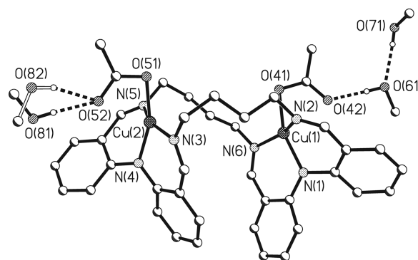
Figure 6. Perspective view of [\text{Cu}^{\text{II}}_2\text{L}^{\text{Pr}}(\text{OAc})_2] \cdot 3\text{MeOH} . Hydrogen atoms, other than those involved in hydrogen bonds, are omitted for clarity.
