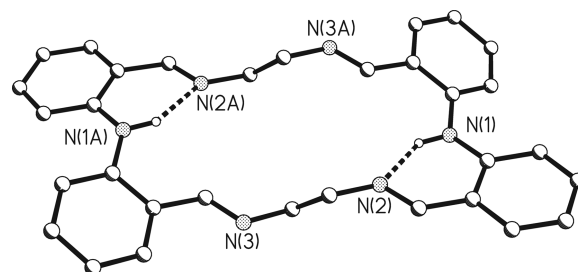
Figure 2. Perspective view of H_2L^{Et} . The second half of the molecule is generated by an inversion operation ( -x, 1-y, -z ). Hydrogen atoms, other than those involved in hydrogen bonds, are omitted for clarity. N(1) \cdots N(2) 2.7113(13) Å.
