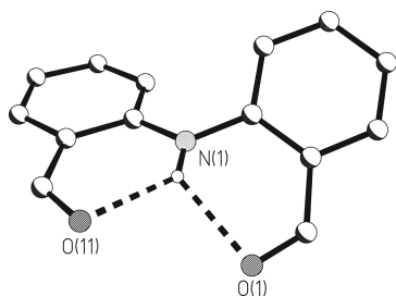
Figure 1. Perspective view of 2,2'-iminobisbenzaldehyde. Hydrogen atoms (except H1x) have been omitted for clarity. N(1) \cdots O(1) 2.7707(18) Å; N(1) \cdots O(11) 2.7510(17) Å. O(1) \cdots H(1X) \cdots O(11) 99.7(8)°.
