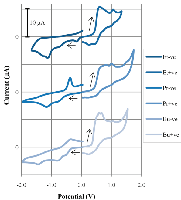
Figure 9. CVs of copper(II) tetrafluoroborate macrocyclic complexes 4 , 5 , and 6 run at 200 \text{ mV/s} in MeCN versus Ag/ 0.01 \text{ mol} \cdot \text{L}^{-1} \text{ AgNO}_3 . Shown are two separate scans per complex, both starting from 0 V but one initially scanning to negative potentials and the other to positive potentials.
