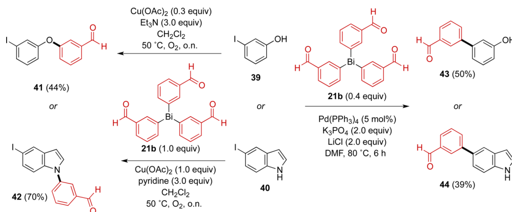
Scheme 9. Orthogonal C-, N-Arylation and O-Arylation of 3-Iodophenol 39 and 5-Iodoindole 40 Using Triis(3-formylphenyl)bismuthine 21b
