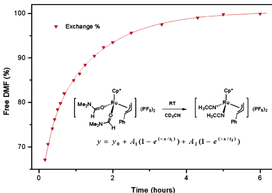
Figure 6. Solvent exchange of the bis-DMF complex [\text{RuCp}^*(\eta^3\text{-CH}_2\text{-CH-CHPh})(\text{DMF})_2](\text{PF}_6)_2 , 4b , to afford the bis-acetonitrile complex [\text{RuCp}^*(\eta^3\text{-CH}_2\text{-CH-CHPh})(\text{CH}_3\text{CN})_2](\text{PF}_6)_2 , 4a . Salt 4b was dissolved in \text{CD}_3\text{CN} , and the appearance of free DMF was monitored by ^1\text{H} NMR spectroscopy ( y_0 = 57.16157 ; A_1 = 13.68922 ; t_1 = 0.2404 ; A_2 = 29.50985 ; t_2 = 1.37759 ).
