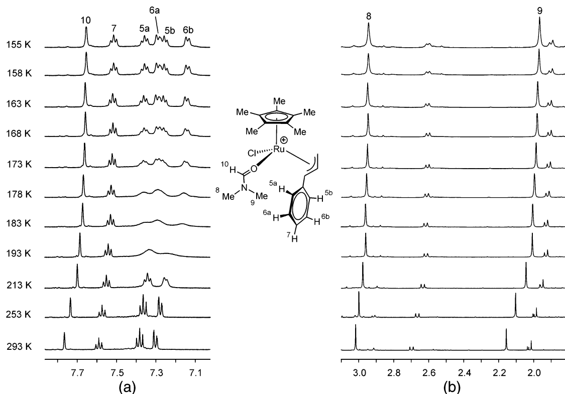
Figure 7. Variable-temperature ^1\text{H} NMR spectra for a sample of 2b . The change in the aromatic region (a) stems from the restricted rotation around the C( ipso )-C(Ph) bond, whereas the pronounced low-frequency shift of one of the DMF methyl groups (b) is assigned to an anisotropic effect (500 MHz, \text{CD}_2\text{Cl}_2 ).
