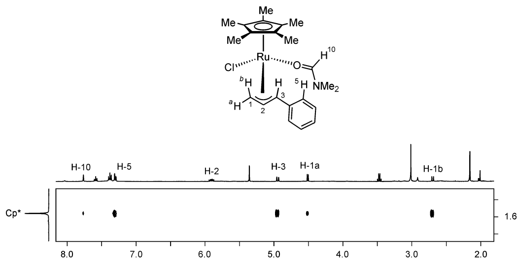
Figure 1. Section of the phase-sensitive ^1\text{H} , ^1\text{H} NOESY spectrum of 2b at ambient temperature, showing the relatively strong contacts from the Cp* methyl groups to the terminal allyl anti protons H-1b and H-3. There is also a modest contact to the syn allyl proton H-1a and no contact to the central allyl proton. These data suggest that the endo configuration is the correct structure ( \text{CD}_2\text{Cl}_2 , 500 MHz).
