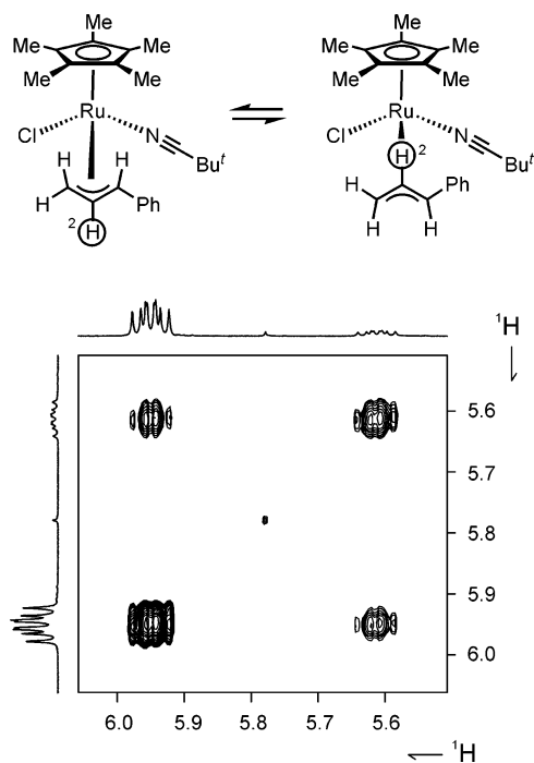
Figure 2. Section of the ^1\text{H} , ^1\text{H} phase-sensitive NOESY spectrum of 2c at ambient temperature showing the exchange between the central allyl proton H-2 of the two isomers ( \text{CD}_2\text{Cl}_2 , 500 MHz).
