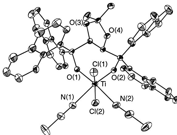
Fig. 6. ORTEP View (30% probability ellipsoids) of [\text{TiCl}_2(1\text{-Nph-TADDOLato})(\text{MeCN})_2] \cdot \text{CH}_2\text{Cl}_2 ( 4b ). H-Atoms and solvent of crystallization are omitted for clarity.
