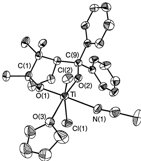
Fig. 7. ORTEP View (30% probability ellipsoids) of [\text{TiCl}_2(\mathbf{13a-ato})(\text{THF})(\text{MeCN})] \cdot \text{MeCN} ( 14 )
