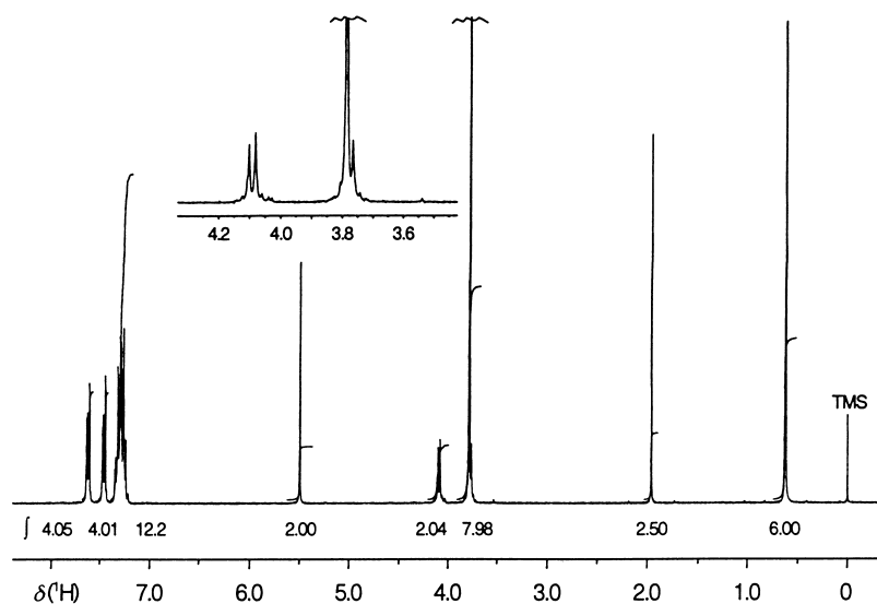
Fig. 1. ^1\text{H} -NMR (300 MHz, \text{CDCl}_3 ) of [\text{TiCl}_2(\text{TADDOLato})(\text{DME})] \cdot \text{MeCN} ( 3 )
