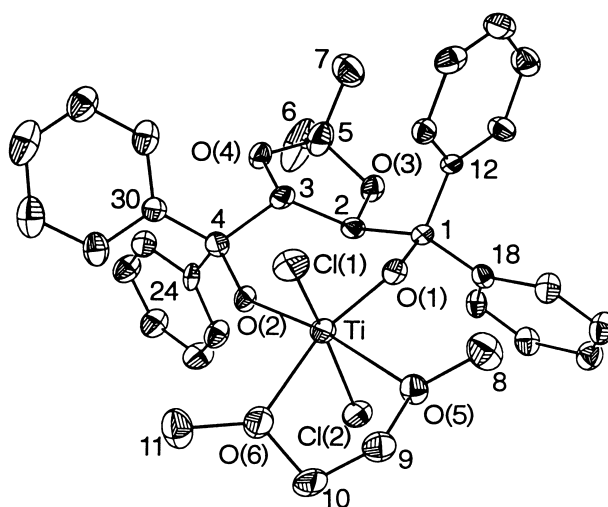
Fig. 5. ORTEP View (30% probability ellipsoids) of the unique independent complex molecule in [\text{TiCl}_2(\text{TADDOLato})(\text{DME})] \cdot \text{MeCN} ( 3 ). H-Atoms and solvent of crystallization are omitted. C-Atoms are numbered without bearing atom symbols.
