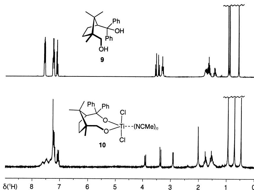
Fig. 3. ^1\text{H} -NMR (300 MHz, \text{CDCl}_3 ) Spectra of diol 9 and the in situ formed complex 10
