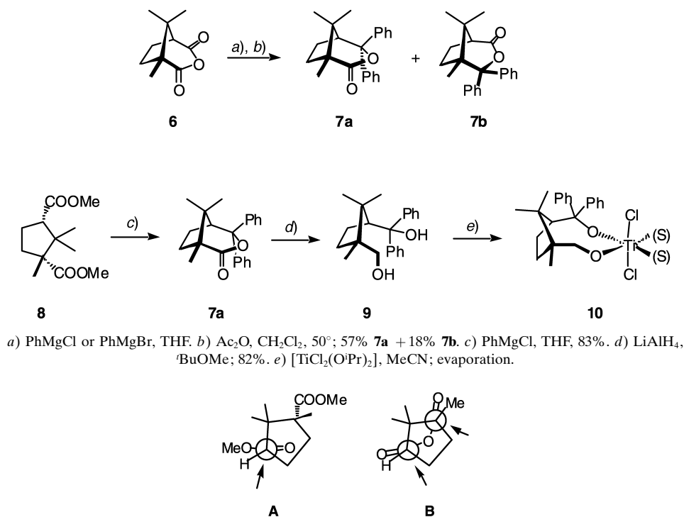
Fig. 2. Regioselectivity of the PhMgCl attack rationalized by the Felkin-Ahn model: A from 8 and B from 6
