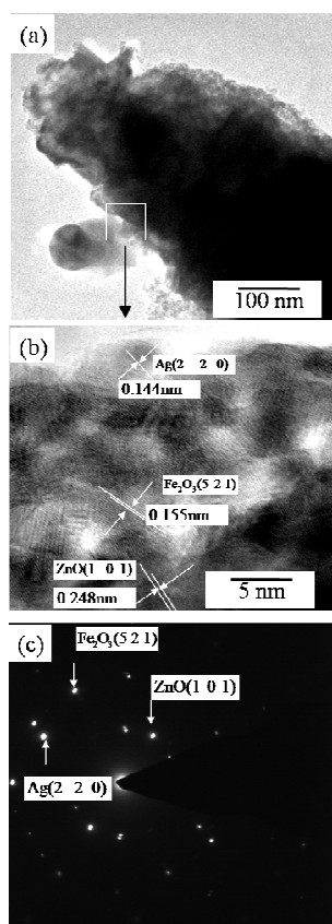
Fig. 3 (a) TEM image of the \text{Ag}/\text{Fe}_2\text{O}_3/\text{ZnO} ternary composite, (b) HR-TEM image of the area indicated by white rectangle in (a), and (c) the SAED pattern of (a).
