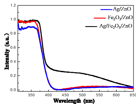
Fig. 5 UV-vis absorption spectra of \text{Ag}/\text{ZnO} , \text{Fe}_2\text{O}_3/\text{ZnO} and \text{Ag}/\text{Fe}_2\text{O}_3/\text{ZnO} .
