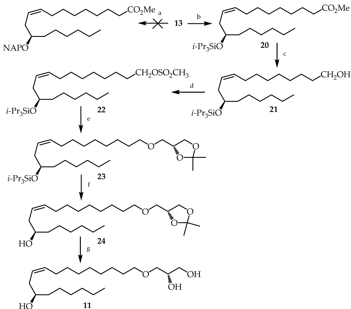
Scheme 2. Synthesis of AKG 11 . Reagents and conditions: (a) 2-(bromomethyl)naphthalene, NaOH, n -Bu 4 NBr, DMSO, 18 h, rt; (b) ClSi i -Pr 3 , imidazole, DMF, 48 h, rt, 61%; (c) Red-Al, Et 2 O, 0 °C, 5 h, 94%; (d) MsCl, Et 3 N, DCM, −50 °C, 2 h, 76%; (e) 18 , NaH, DMF, 15 h, rt, 68%; (f) TBAF, THF, rt, 20 h, 92%; (g) p -TsOH·H 2 O (0.05 equiv), MeOH/H 2 O (9:1), 60 °C, 4 h, 84%.
