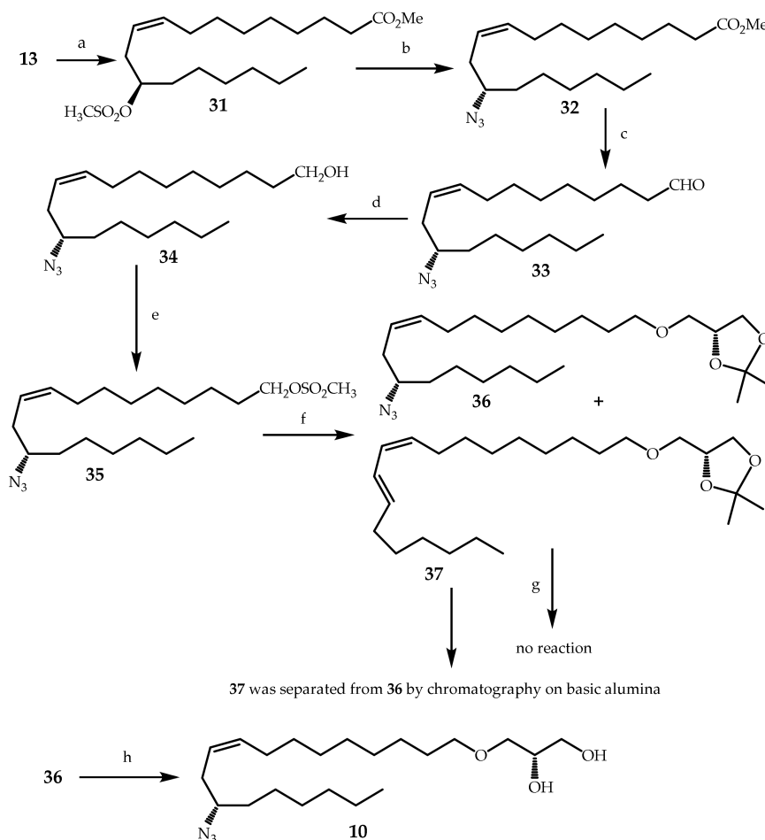
Scheme 4. Synthesis of AKG 10 . Reagents and conditions: (a) \text{MsCl} , \text{Et}_3\text{N} , DCM, -10\text{ }^\circ\text{C} , 4 h, 65%; (b) \text{NaN}_3 , DMSO, 80\text{ }^\circ\text{C} , 18 h, 80%; (c) Dibal, \text{Et}_2\text{O} , -80\text{ }^\circ\text{C} , 2 h, 68%; (d) \text{NaBH}_4 , EtOH, 0\text{ }^\circ\text{C} , 1 h, 74%; (e) \text{MsCl} , \text{Et}_3\text{N} , DCM, -50\text{ }^\circ\text{C} , 4 h and then up to -5\text{ }^\circ\text{C} , 59%; (f) 18 , 50% aqueous NaOH, n - \text{Bu}_4\text{NBr} , DMSO, 40\text{ }^\circ\text{C} , 15 h; (g) maleic anhydride, cyclohexane, 72 h, 45\text{ }^\circ\text{C} ; (h) p - \text{TsOH}\cdot\text{H}_2\text{O} (0.05 equiv), MeOH/ \text{H}_2\text{O} (9:1), 60\text{ }^\circ\text{C} , 5 h, 97%.
