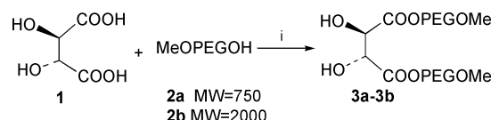
Scheme 1 Reagents and conditions: MeOPEGOH = \text{MeO}-(\text{CH}_2\text{CH}_2\text{O})_n-\text{CH}_2\text{CH}_2\text{OH} ; i, p -toluenesulfonic acid (5 mass%), ca. 115^\circ\text{C} , 45 h.
