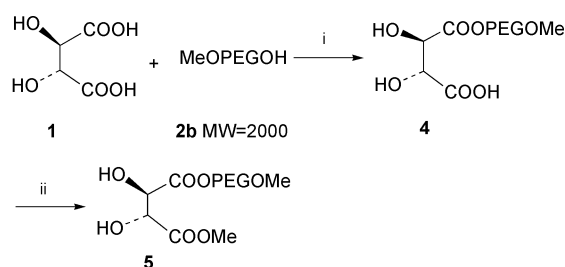
Scheme 2 Reagents and conditions: MeOPEGOH = \text{MeO}-(\text{CH}_2\text{CH}_2\text{O})_n-\text{CH}_2\text{CH}_2\text{OH} ; i, p -toluenesulfonic acid (5 mass%), ca. 115^\circ\text{C} , 45 h; ii, \text{CH}_2\text{N}_2 , rt.
