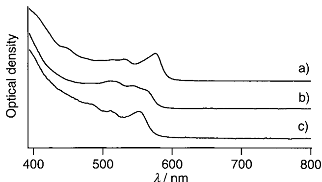
Fig. 5. Qualitative comparison of the absorption spectra ( CH_2Cl_2 , 20°) of a) hexakis-adduct ( \pm )- 1 , b) heptakis-adduct ( \pm )- 30 , and c) octakis-adduct ( \pm )- 31 . The molar extinction coefficients of ( \pm )- 30 and ( \pm )- 31 were not determined due to the small quantity of material.
