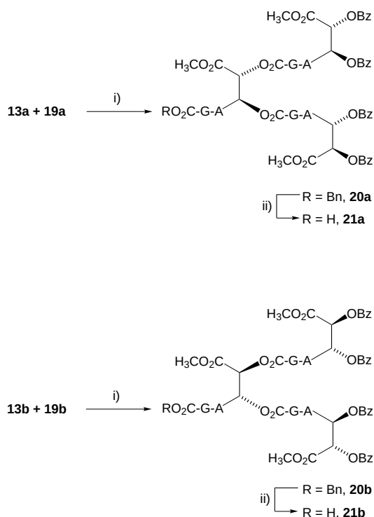
Scheme 6. Syntheses of the second-generation dendra 21a,b : i) dioxane, DCC, DMAP, 60–65 %; ii) dioxane, \text{H}_2 , Pd-C, 100 %.
