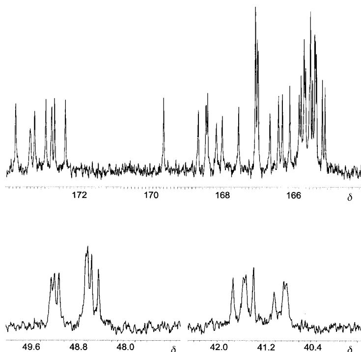
Figure 2. ^{13}\text{C} NMR spectrum (125.7 MHz, \text{CDCl}_3 ) of 22a for the ranges from \delta = 164\text{--}174 ( \text{C}=\text{O} ), \delta = 46\text{--}50 (CH alanine), and \delta = 40\text{--}42 ( \text{CH}_2 glycine).
