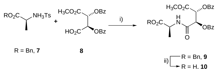
Scheme 2. Synthesis of the acid 10 : i) \text{NEt}_3 , DCC, \text{CH}_2\text{Cl}_2 , 0^\circ\text{C} , 52%; ii) dioxane, \text{H}_2 , Pd-C, 100%. Bn = benzyl, Bz = benzoyl.
