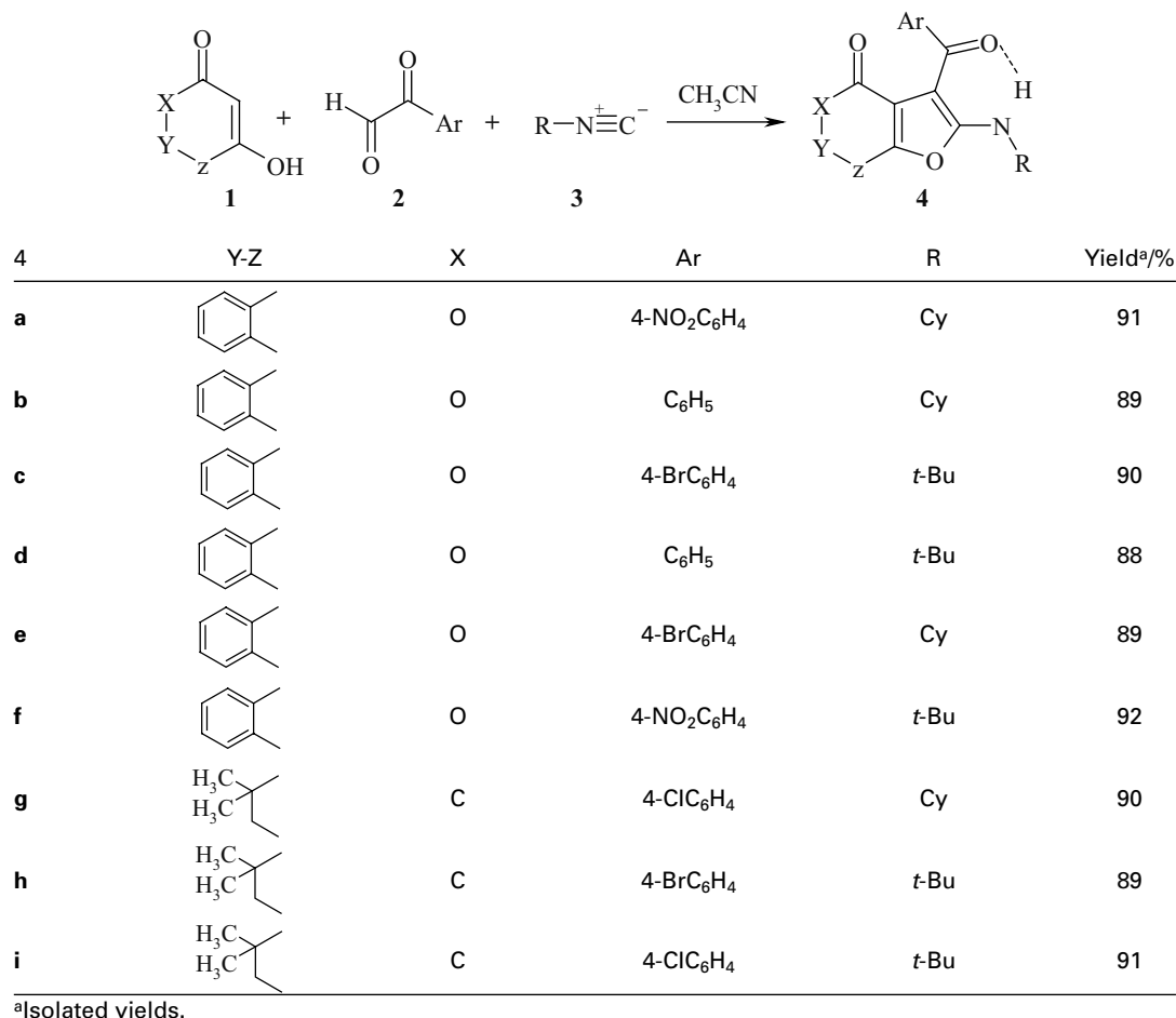
Scheme 1 Three-component reaction between 4-hydroxycoumarin or 5,5-dimethyl-1,3-cyclohexandione, arylglyoxals and isocyanides.
