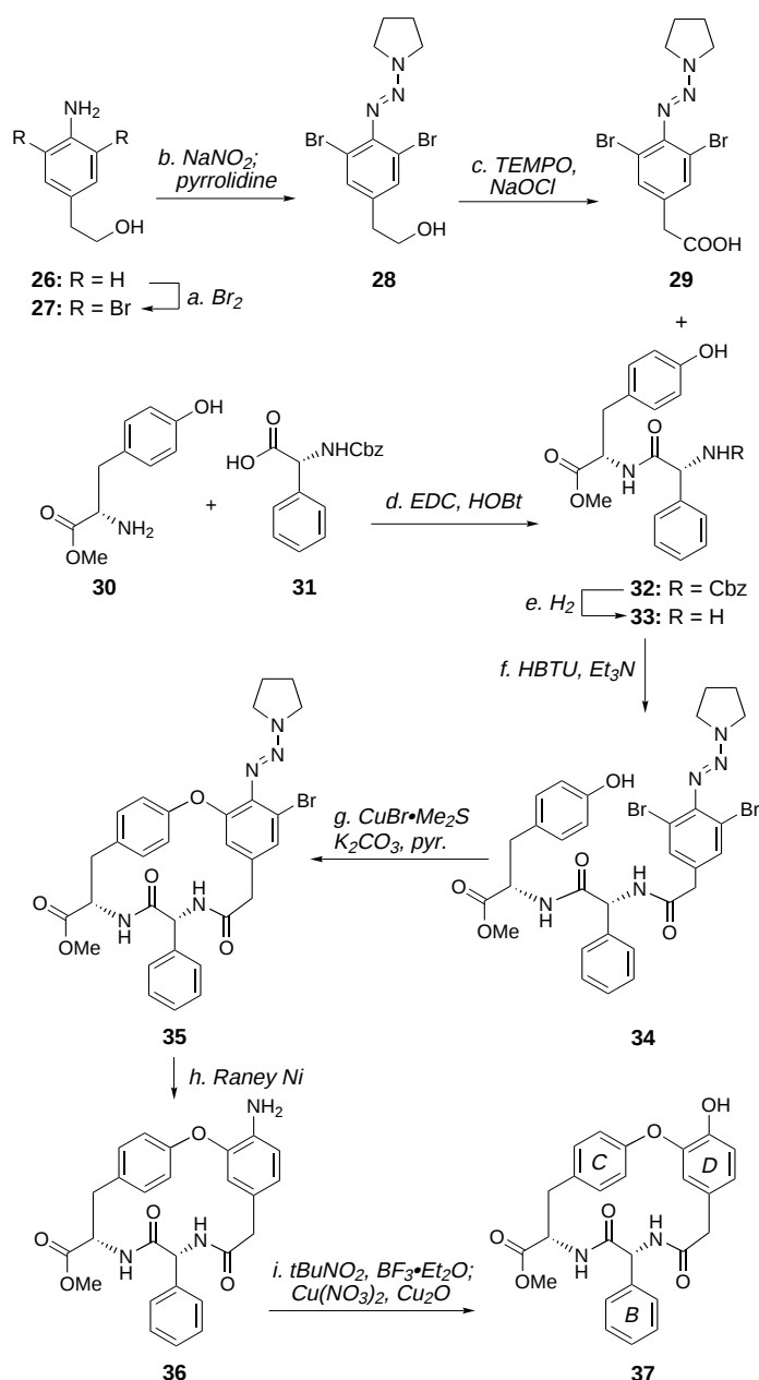
Scheme 2. Synthesis of C-O-D model system 37 . a) 2.2 equiv of Br 2 , AcOH, 25 °C, 0.5 h, 99%; b) 1.3 equiv of NaNO 2 , 5.0 equiv of 12 N aq HCl, THF/H 2 O (10:1), 0 °C, 0.5 h; then 10.0 equiv of pyrrolidine, sat. aq K 2 CO 3 , 0 °C, 1 h, 84%; c) 1.5 equiv of TEMPO, 3.0 equiv of 5% aq NaOCl, 10 mol % of KBr, acetone/5% NaHCO 3 (1:1), 0 °C, 2 h, 82%; d) 1.5 equiv of EDC, 1.5 equiv of HOBT, DMF, 0 °C, 10 h, 91%; e) H 2 , 10% Pd/C, MeOH, 25 °C, 1 h, 100%; f) 1.5 equiv of HBTU, 2.0 equiv of 33 , 1.5 equiv of Et 3 N, DMF, 0 °C, 18 h, 63%; g) 2.5 equiv of K 2 CO 3 , 2.5 equiv of CuBr·Me 2 S, 3.0 equiv of pyr., MeCN (0.01 M), 75 °C, 15 h, 77%; h) Raney Ni, MeOH, reflux, 2 h, 71%; i) 1.5 equiv of t BuNO 2 , 3.0 equiv of BF 3 ·Et 2 O, THF, −20 → 5 °C, 0.5 h; then sat. Cu(NO 3 ) 2 , 5.0 equiv of Cu 2 O, H 2 O, 25 °C, 3 h, 60%. DMF = dimethylformamide; EDC = 1-ethyl-3-(3-dimethylamino)-propyl carbodiimide hydrochloride; HOBT = 1-hydroxybenzotriazole; TEMPO = 2,2,6,6-tetramethyl-1-piperidinyloxy; HBTU = 2-(1 H -benzotriazole-1-yl)-1,1,3,3-tetramethyluronium hexafluorophosphate; Cbz = benzyloxycarbonyl.
