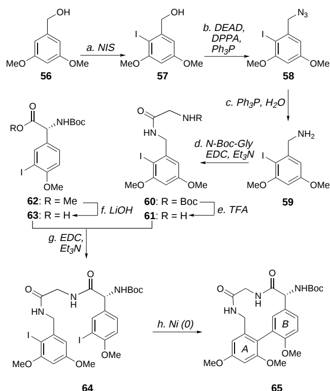
Scheme 6. Construction of model AB biaryl system 65 by nickel (0)-mediated coupling reaction. a) 1.5 equiv of NIS, DMF, 25 °C, 12 h, 91%; b) 1.5 equiv of \text{Ph}_3\text{P} , 1.5 equiv of DEAD, 1.5 equiv of DPPA, THF, 0 °C, 2 h, 82%; c) 3.0 equiv of \text{Ph}_3\text{P} , THF/ \text{H}_2\text{O} (10:1), 45 °C, 4 h, 80%; d) 1.0 equiv of N -Boc-Gly, 1.5 equiv of EDC, 2.5 equiv of \text{Et}_3\text{N} , DMF, 0 °C, 12 h, 81%; e) TFA/ \text{CH}_2\text{Cl}_2 (1:1), 0 \rightarrow 25 °C, 2 h, 100%; f) 1.5 equiv of LiOH, THF/ \text{H}_2\text{O} (1:1), 0 °C, 1 h, 99%; g) 1.2 equiv of 63 , 1.3 equiv of EDC, 2.2 equiv of \text{Et}_3\text{N} , DMF, 0 °C, 12 h, 92%; h) 1.8 equiv of (\text{Ph}_3\text{P})_2\text{NiCl}_2 , 1.8 equiv of Zn, 3.6 equiv of \text{Ph}_3\text{P} , DMF (0.002 M), 55 °C, 16 h, ca. 1:1 ratio of atropisomers, 26% combined yield. NIS = N -iodosuccinimide; TFA = trifluoroacetic acid.
