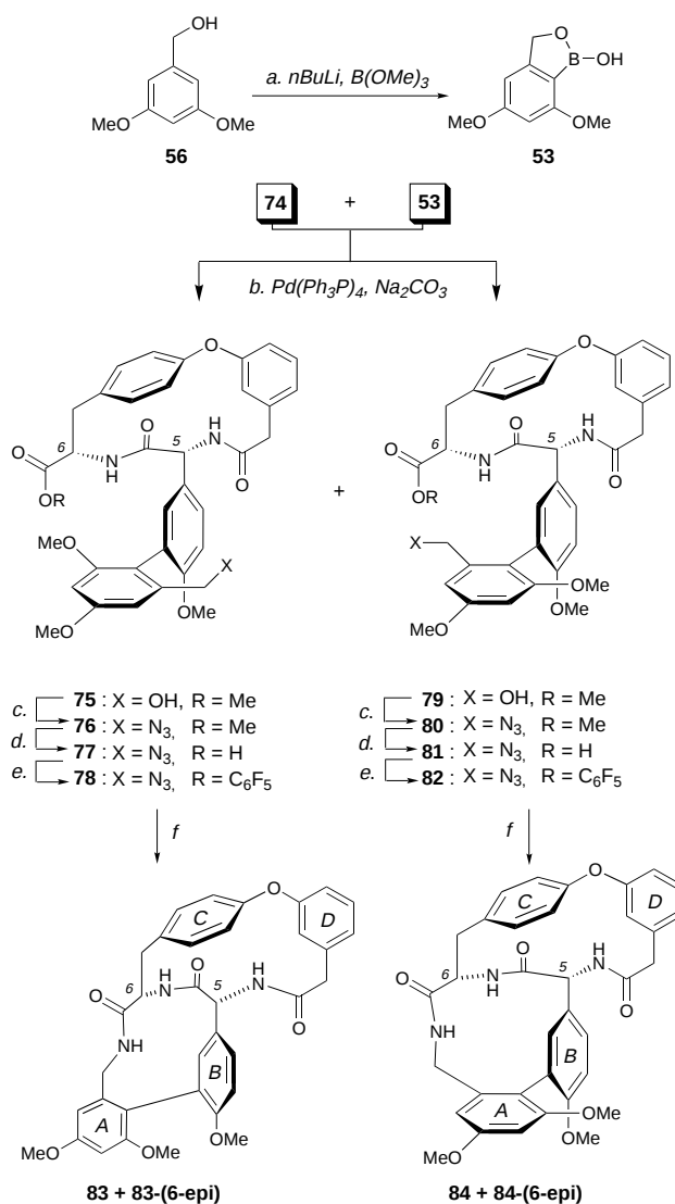
Scheme 8. Construction of AB/C-O-D model bicyclic systems 83 and 84 by the Suzuki–macrolactamization strategy. a) 2.2 equiv of n BuLi, benzene, 0 °C, 2 h; then 3.0 equiv of \text{B}(\text{OMe})_3 , THF, -78 \rightarrow -25 °C, 6 h, 5 % aq HCl, 46 %; b) 10 mol % of \text{Pd}(\text{PPh}_3)_4 , 1.0 equiv of \text{Na}_2\text{CO}_3 , toluene/MeOH/ \text{H}_2\text{O} (80:18:2), 90 °C, 2 h, 75 : 79 ca. 1:1, 80 % combined yield; c) 5.0 equiv of \text{HN}_3 , 5.0 equiv of DEAD, 5.0 equiv of \text{Ph}_3\text{P} , THF, 0 \rightarrow 25 °C, 1 h, 69 %; d) 1.5 equiv of LiOH, THF/ \text{H}_2\text{O} (1:1), 0 °C, 0.5 h, 100 %; e) 2.0 equiv of \text{C}_6\text{F}_5\text{OH} , 1.2 equiv of DCC, 0.2 equiv of 4-DMAP, \text{CH}_2\text{Cl}_2 , 25 °C, 1 h; f) 3.0 equiv of 4-pyrrolidinopyridine, 0.3 equiv of 10 % Pd/C, dioxane/ethanol/cyclohexene (90:8:2), 0.001 M, 90 °C, 5 h, 30 % from 77 and 81 . \text{C}_6\text{F}_5\text{OH} = pentafluorophenol; DCC = N,N' -dicyclohexylcarbodiimide; 4-DMAP = 4-dimethylaminopyridine.
