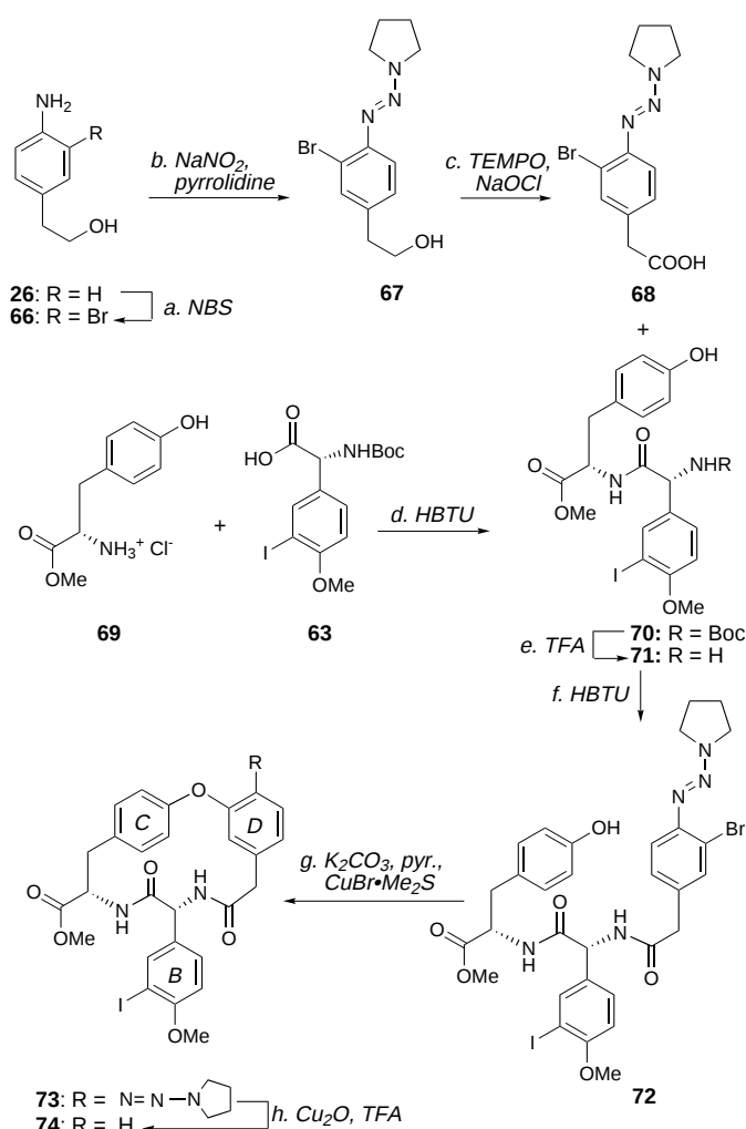
Scheme 7. Construction of model C-O-D template 74 . a) 1.2 equiv of NBS, DMF, 25 °C, 12 h, 62%; b) 1.2 equiv of conc. aq. HCl, 1.0 equiv of \text{NaNO}_2 , 0 °C, 0.5 h; then sat. aq. \text{K}_2\text{CO}_3 , 10.0 equiv of pyrrolidine, 0 °C, 1 h, 83%; c) 1.0 equiv of TEMPO, 0.1 equiv of KBr, 1.3 equiv of NaOCl, acetone:5% \text{NaHCO}_3 (1:1), 0 °C, 1.5 h, 86%; d) 1.2 equiv of HBTU, 3.0 equiv of \text{Et}_3\text{N} , DMF, 0 \rightarrow 25 °C, 3 h, 90%; e) TFA: \text{CH}_2\text{Cl}_2 (1:1), 0 °C, 1 h, 100%; f) 1.2 equiv of HBTU, 3.0 equiv of \text{Et}_3\text{N} , DMF, 0 \rightarrow 25 °C, 3 h, 90%; g) 2.9 equiv of \text{CuBr}\cdot\text{Me}_2\text{S} , 2.4 equiv of \text{K}_2\text{CO}_3 , 3.0 equiv of pyr., MeCN, reflux, 36 h, 67% (10% recovered 72 and 6% arylglycine epimer of 73 ); h) 2.2 equiv of TFA, 5.0 equiv of \text{Cu}_2\text{O} , THF, reflux, 1 h, 90%. NBS = N -bromosuccinimide.
