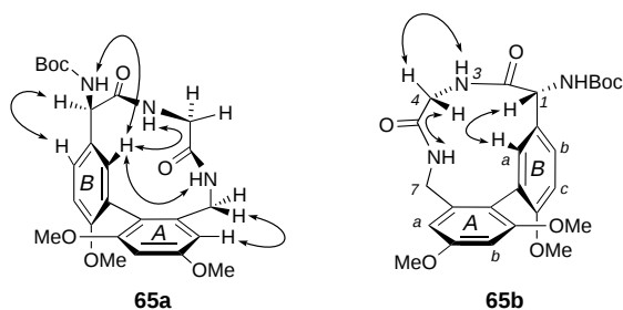
Figure 2. Assignments of stereochemistry of atropisomers 65a and 65b by ^1\text{H} - ^1\text{H} NOE studies (COSY, NOESY, \text{CDCl}_3 , 600 MHz).
