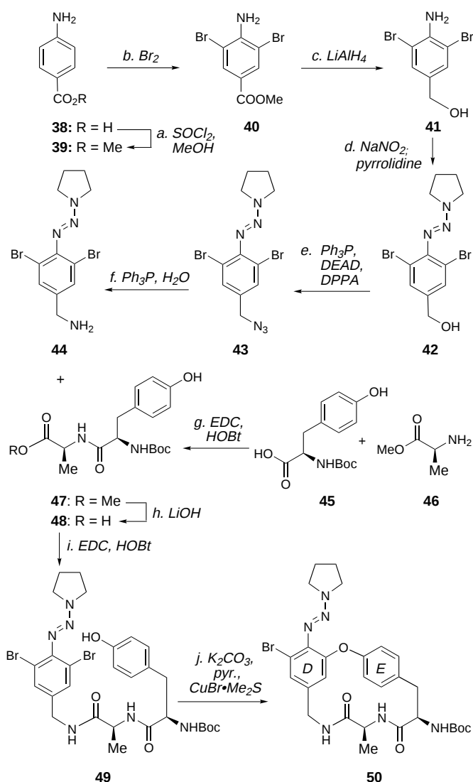
Scheme 3. Synthesis of D-O-E model system 50 . a) 1.1 equiv of SOCl 2 , MeOH, reflux, 2 h, 98%; b) 2.2 equiv of Br 2 , AcOH, 25 °C, 0.5 h, 99%; c) 3.0 equiv of LiAlH 4 , THF, 0 °C, 4 h, 93%; d) 1.3 equiv of NaNO 2 , 5.0 equiv of 12 N aq HCl, THF/H 2 O (10:1), 0 °C, 0.5 h; then 10.0 equiv of pyrrolidine, sat. aq K 2 CO 3 , 0 °C, 1 h, 73%; e) 1.5 equiv of Ph 3 P, 1.5 equiv of DEAD, 1.5 equiv of DPPA, THF, 25 °C, 2 h, 82%; f) 2.0 equiv of Ph 3 P, 10.0 equiv of H 2 O, THF, 45 °C, 8 h, 80%; g) 1.5 equiv of EDC, 1.5 equiv of HOBT, DMF, 0 °C, 8 h; h) 1.5 equiv of LiOH, MeOH/H 2 O (1:1), 0 °C, 1 h, 85% from 45 ; i) 1.5 equiv of 48 , 3.0 equiv of EDC, 1.5 equiv of HOBT, DMF, 0 °C, 8 h, 45%; j) 2.5 equiv of K 2 CO 3 , 2.5 equiv of CuBr·Me 2 S, 3.0 equiv of pyr., MeCN (0.01 M), 75 °C, 6 h, 54% (87% conversion). DEAD = diethyl azodicarboxylate; DPPA = diphenylphosphoryl azide; Boc = t -butoxycarbonyl.
