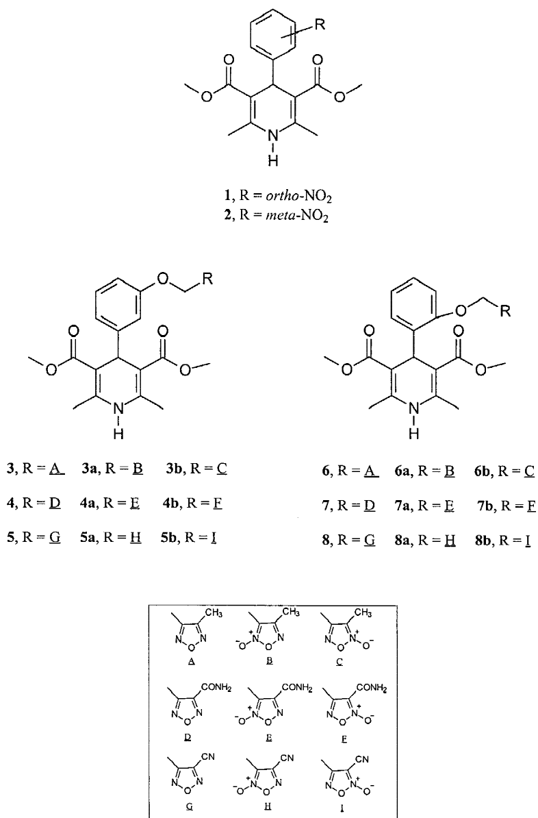
Fig. 1. Nitrosubstituted 1,4-DHPs and related furazan and furoxan derivatives.
