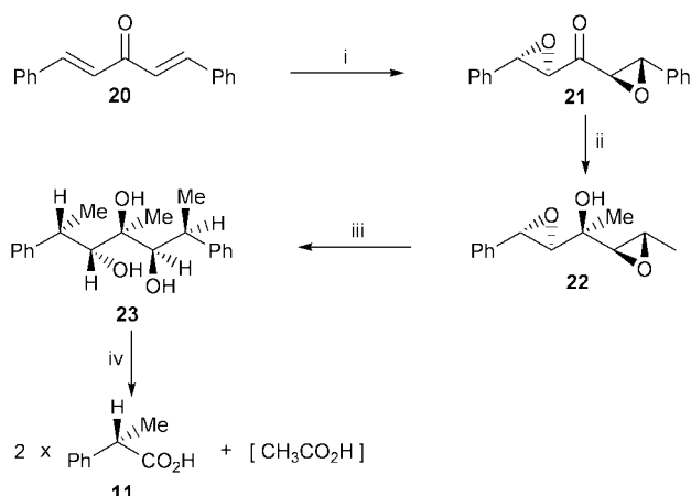
Scheme 2 Reagents and conditions (yields in parenthesis): (i) Poly-(L)-leucine adsorbed onto silica, tert -butyl methyl ether containing urea-hydrogen peroxide and DBU, -10^{\circ}\text{C} (90%); (ii) MeMgI, THF, Et 2 O, -78^{\circ}\text{C} (88%); (iii) Me 3 Al, hexane, -78^{\circ}\text{C} (71%); (iv) NaIO 4 /SiO 2 , CH 2 Cl 2 ; then Jones oxidation (69%).
