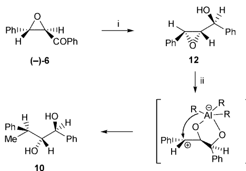
Scheme 1 Reagents and conditions (yields in parenthesis): (i) \text{Zn}(\text{BH}_4)_2 (0.3 equiv.), \text{Et}_2\text{O} , 0 °C, 30 min (95%); (ii) \text{Me}_3\text{Al} (3 equiv.), hexane, 0 °C (93%).
