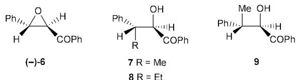
Scheme 1 Reagents and conditions (yields in parenthesis): (i) \text{Zn}(\text{BH}_4)_2 (0.3 equiv.), \text{Et}_2\text{O} , 0 °C, 30 min (95%); (ii) \text{Me}_3\text{Al} (3 equiv.), hexane, 0 °C (93%).
