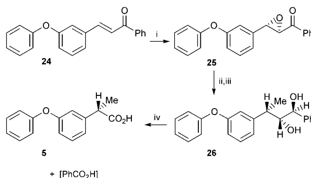
Scheme 3 Reagents and conditions (yields in parenthesis): (i) Poly-(L)-leucine adsorbed onto silica, urea-hydrogen peroxide, DBU, THF, 2 h (98% yield, 94% ee); (ii) Zn(NH 4 ) 2 (0.3 equiv.), Et 2 O, 0^{\circ}\text{C} , 3 h (95%); (iii) Me 3 Al (3 equiv.), hexane, -78^{\circ}\text{C} , 2 h (85%); (iv) NaIO 4 /SiO 2 , CH 2 Cl 2 ; then Jones oxidation (64%).
