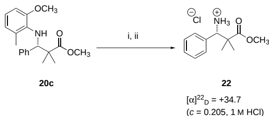
Scheme 6. Oxidative cleavage of the N -aryl substituent from \beta -amino acid 20c . i) 5 equiv \text{CAN} , 0^\circ\text{C} to 22^\circ\text{C} ; ii) \text{Et}_2\text{O} , 56% \text{HCl} .
