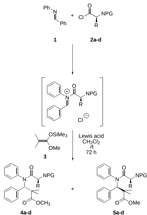
Scheme 1. Asymmetric Mannich reactions via N -acyliminium intermediates employing different N -protected amino acids as chiral auxiliaries.
