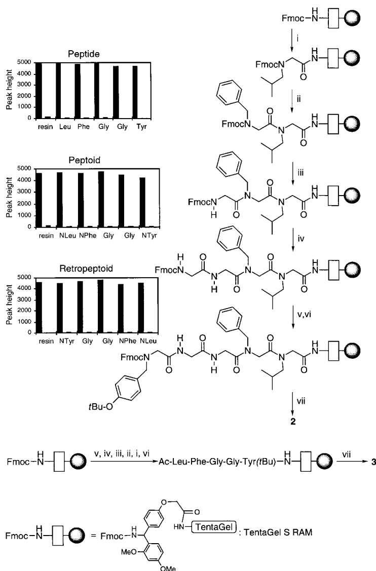
Scheme 3. Solid-phase synthesis of the peptoid 2 and retropeptoid 3 of Leu-enkephalin ( 1 ) and the solid-phase synthesis monitoring profiles. i) a) piperidine, b) Fmoc-NLeu-OH 10b , PyBroP, DiPEA; ii) a) piperidine, b) Fmoc-NPhe-OH 10a , PyBroP, DiPEA; iii) a) piperidine, b) Fmoc-Gly-OH, PyBroP, DiPEA; iv) a) piperidine, b) Fmoc-Gly-OH, PyBroP, DiPEA; v) a) piperidine, b) Fmoc-NTyr( t Bu)-OH ( 10f ), PyBroP, DiPEA; vi) a) piperidine, b) Ac 2 O, DiPEA, HOBT; vii) TFA/H 2 O/TIS, 95/2.5/2.5 (v/v).
