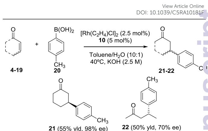
Scheme 3. Pseudo-enantiomeric behavior of ligands 3 and 10 in the Rh-catalyzed 1,4-addition
