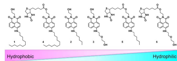
Fig. 2 Lipophilicity of probes (1-6) according to logP oct value.
