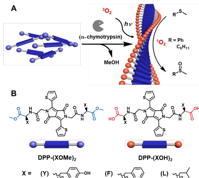
Figure 1. Visible-light photooxidation enabled by a supramolecular hydrogel. (A) Biocatalytic self-assembly of the LMWGs into superstructures via in situ enzymatic hydrolysis of DPP-(XOMe) 2 with \alpha -chymotrypsin. These superstructures were used for the photooxidation of thioanisole and cyclohexyl methyl sulfide via ^1\text{O}_2 formation in water. (B) Photoactive precursors, DPP-(XOMe) 2 and components, DPP-(XOH) 2 , of the supramolecular hydrogels.
