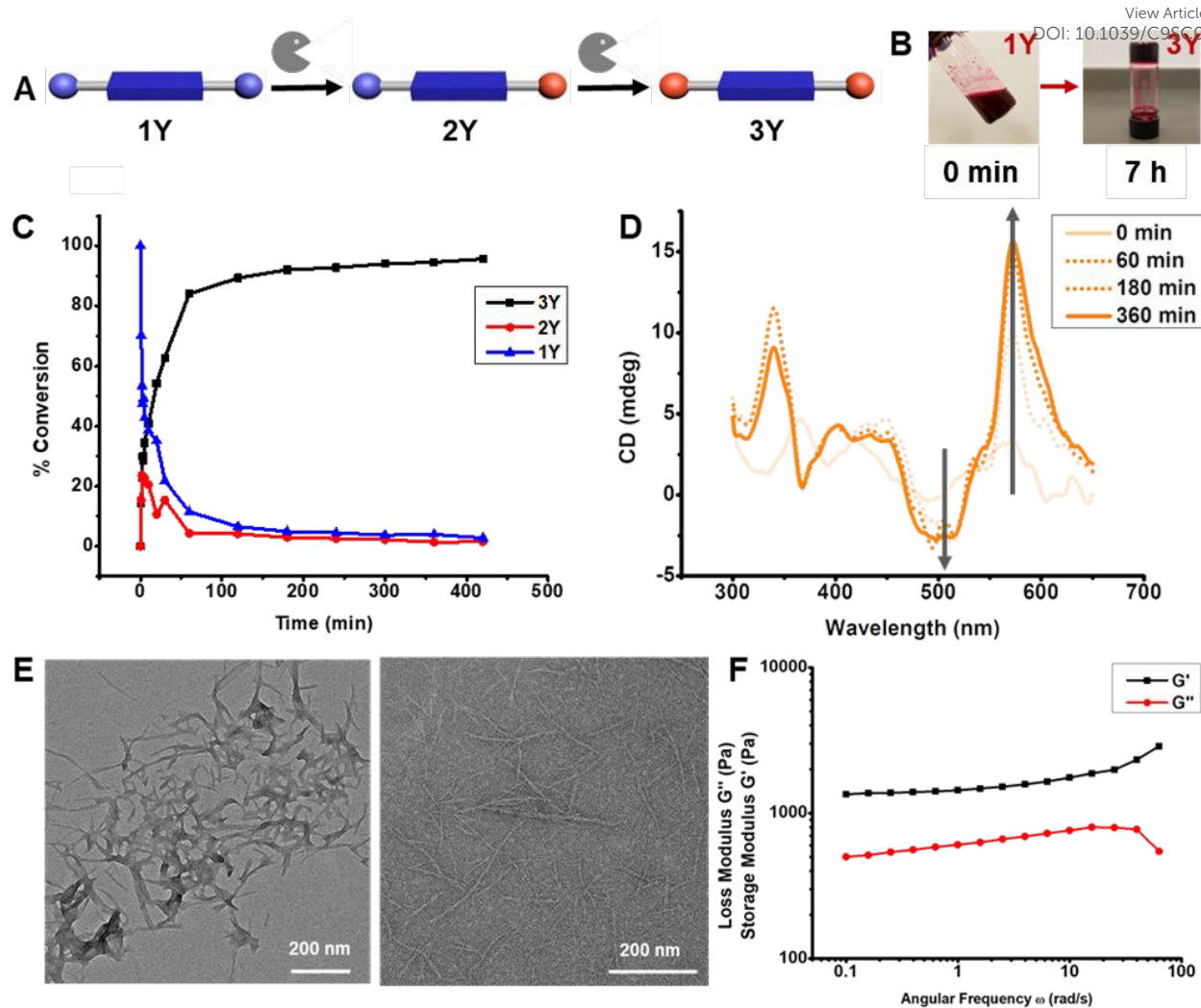
Figure 2. (A) Sequential enzymatic hydrolysis of DPP-(YOMe) 2 in phosphate buffer (pH 8, 100 mM, 5% DMSO) in the presence of \alpha -chymotrypsin (1 mg mL -1 ). (B) Photograph of reaction vial at 0 min (left) and 7 h (right). (C) HPLC analysis of enzymatic hydrolysis of DPP-(YOMe) 2 at 10 mM. (D) CD spectra showing the formation of homochiral superstructure during the enzymatic hydrolysis of DPP-(YOMe) 2 at 10 mM. (E) TEM images of DPP-(YOMe) 2 (left) and DPP-(YOH) 2 (right). (F) Oscillatory rheology of the DPP-(YOH) 2 (10 mM) gel showing elastic modulus ( G' ) of 1.7 kPa (Angular Frequency = 10 rad/s; Frequency sweep).
