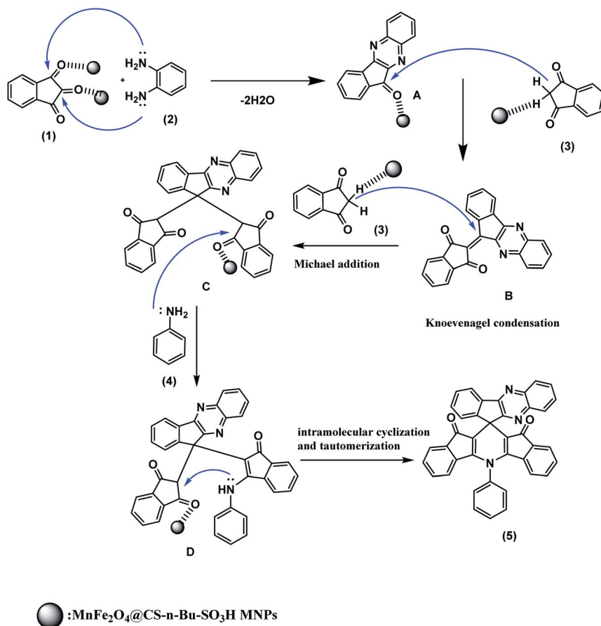
Scheme 2 Plausible mechanism for the synthesis of spiro indenopyridine derivatives.
